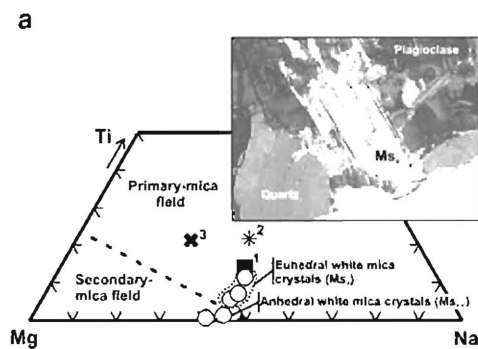
Fig. 6 a Mg–Ti–Na diagram to distinguish between secondary and primary muscovite (Miller et al. 1981). The photomicrograph shows a primary muscovite crystal ( Ms_a ). b Absolute abundance plots of trace elements other than REE in secondary muscovite formed from andalusite and cordierite (average from Table 8). The gray field
