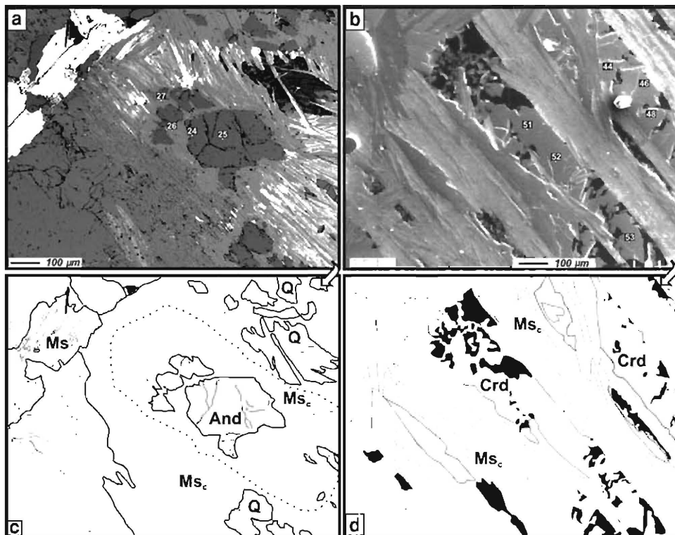
Fig. 3 a, b BSE images with corresponding sketches (c, d) showing the location of electron microprobe spots for andalusite, Na-rich cordierite (Tables 3, 5), muscovite from the Santa Cruz igneous facies and textural relationships among them. According to Clarke et al. (2005), textural relationships like those shown here are indicative of subsolidus replacement of muscovite after andalusite and Na- and Li-rich cordierite that resulted in a polycrystalline muscovite pseudomorph. Mineral abbreviations after Kretz (1983)
