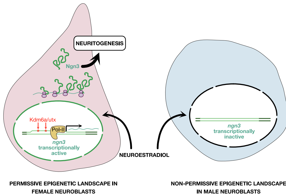
Fig. 4. Role of epigenetic regulation in determining sex-specific actions of neuroestradiol in female neuron neuritogenesis. The X-linked enzyme Kdm6a/Utx, which removes methyl groups in lysine at position 27 of histone H3, exerts an epigenetic regulation of the neuritogenic factor neurogenin 3 (Ngn3) gene, facilitating the upregulation of its transcription by neuroestradiol-activated signaling pathways in developing female neurons.
