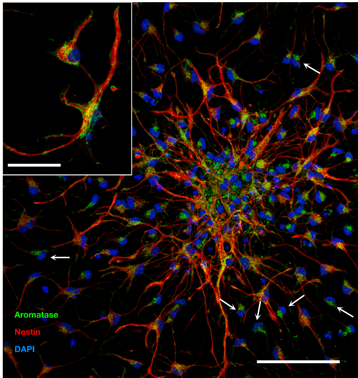
Fig. 2. Aromatase expression in neural stem cells. Aromatase immunoreactivity in a neurosphere derived from P0 mouse hippocampus, plated for 24 h, immunostained for aromatase (green) and the neural stem cell marker nestin (red) and counterstained with the nuclear marker DAPI (blue). Most cells show red and green signals, indicating that neural stem cells express aromatase. The inset show an example of two of these cells that are immunoreactive for aromatase and nestin. Aromatase immunoreactivity shows a reticular aspect corresponding to the localization of the enzyme in the endoplasmic reticulum, while the immunoreactivity for nestin, an intermediate filament, labels the cytoskeleton. Arrows point to aromatase immunoreactive cells that have migrated from the neurosphere and are either nesting negative or show a low level of nestin immunoreactivity, suggesting that they are committed to neuronal differentiation. Scale bar = 50 \mu m; inset, 10 \mu m. (For interpretation of the references to colour in this figure legend, the reader is referred to the web version of this article.)
