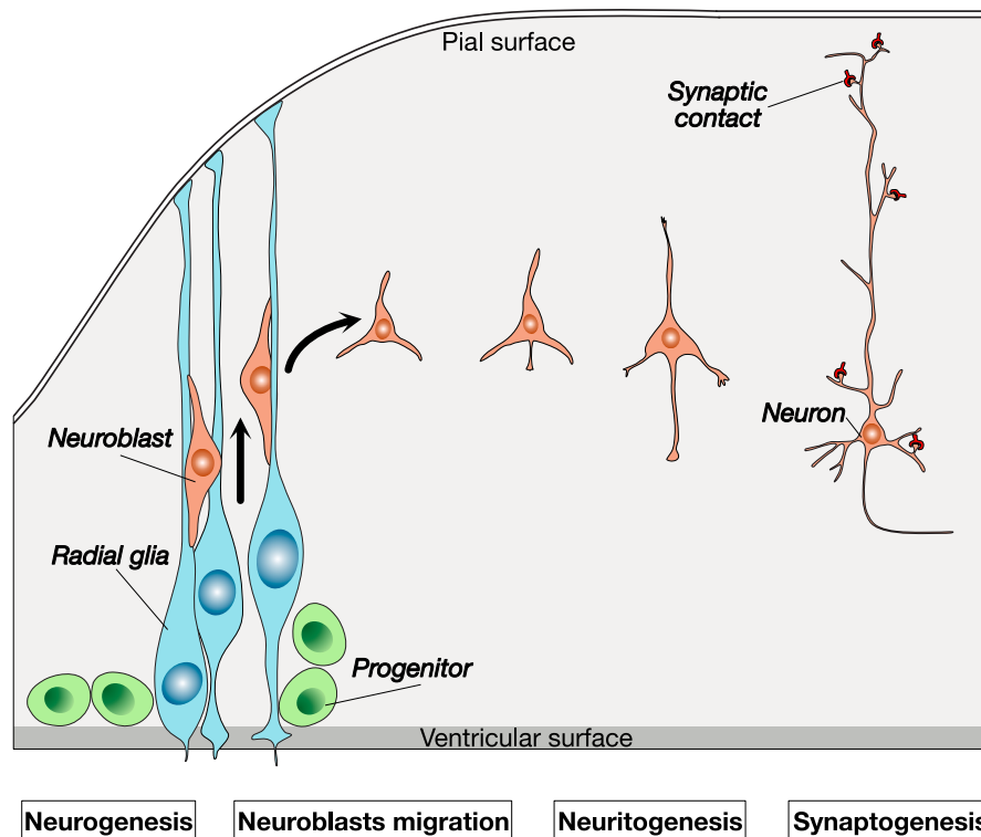
Fig. 1. Neurodevelopmental events that are regulated by neuroestradiol and are discussed in this paper. Aromatase is expressed by progenitor cells, radial glia, migrating neuroblasts and developing neurons. Neuroestradiol regulates neurogenesis, neuroblast migration, neuritogenesis and synaptogenesis in both sexes.
