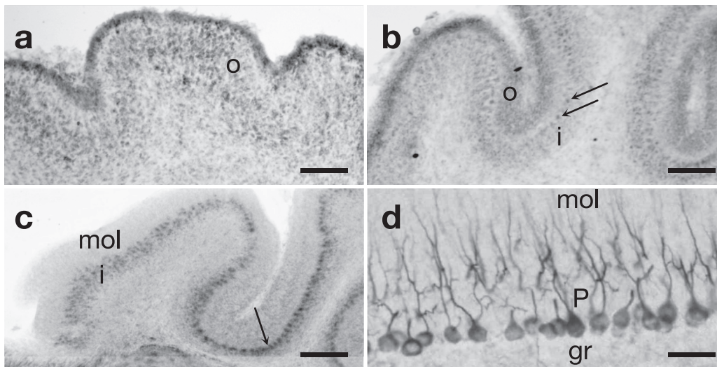
Fig. 3. Transient aromatase immunoreactivity in migrating granule cell neuroblasts in the developing mouse cerebellar cortex. Examples of histological sections of the mouse cerebellar cortex at postnatal developmental stages P2 (a), P4 (b), P7 (c) and P21 (d). The histological sections were immunostained with an antibody raised against mouse aromatase (Garcia-Segura et al., 1999), without counterstaining. a, At postnatal day P2 aromatase immunoreactivity is confined to migrating neuroblast in the outer granular layer (o). b, At P4 migrating neuroblasts have formed an inner granular layer (i), which is separated from the outer (o) granular layer by alienated aromatase-immunoreactive cell bodies of Purkinje cells (arrows). c, At P7 all granule cells have reached the inner granular layer (i) and initiate to turn off aromatase expression, while Purkinje
