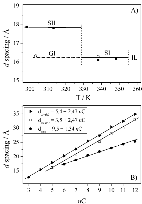
Figure 6. (A) d -Spacing vs temperature for the Pb(C5) 2 phases (■, on heating; ○, on cooling). S II , ordered crystal; S I , rotator phase; G I , S I , glass state; IL, isotropic liquid. (B) d -Spacings vs alkyl chain number of carbons ( n ), for the following: right-pointing solid triangle, crystal phase; □, rotator phase; ●, neat phase.
