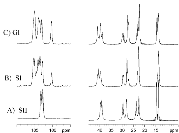
Figure 9. C-13 CP/MAS-NMR spectra of \text{Pb}(\text{C5})_2 : (A) crystalline phase (SII) at room temperature; (B) rotator phase (SI) at 343 K; (C) solidified after being melted (GI) at room temperature.
