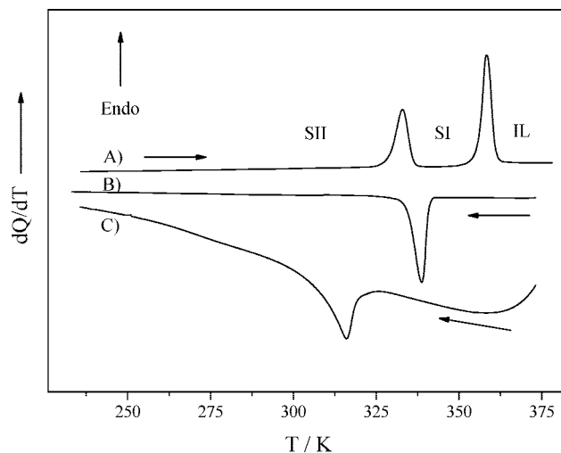
Figure 1. Thermograms of Pb(C5) 2 : (A) first heating at 5 K·min -1 ; (B) cooling at 5 K·min -1 ; (C) cooling fast, at approximately 40 K·min -1 .
