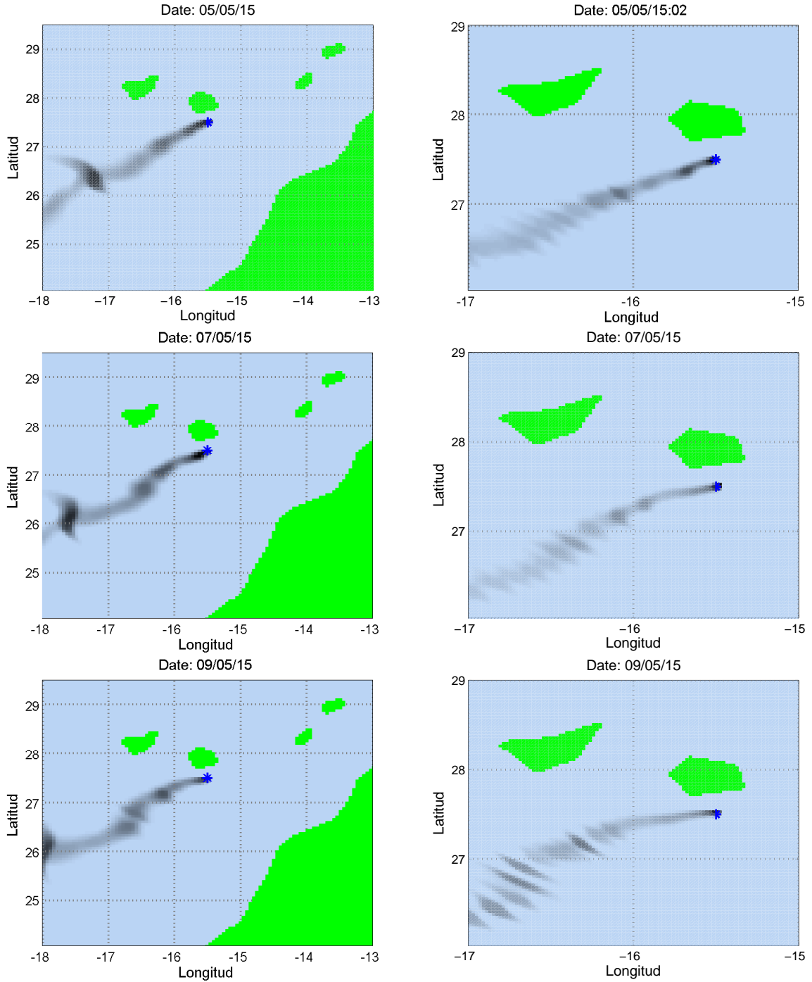
Figure 6: Oil concentration simulated by the model, considering the computational domains (Left) \Omega and (Right) \Omega_z , presented in this work for the dates: (Top) May 5, 2015, (Middle) May 7, 2015 and (Bottom) May 9, 2015. The coast is also represented in green. The position of the Oleg Naydenov ship is represented by a blue star. The drag factor is 0.022.
