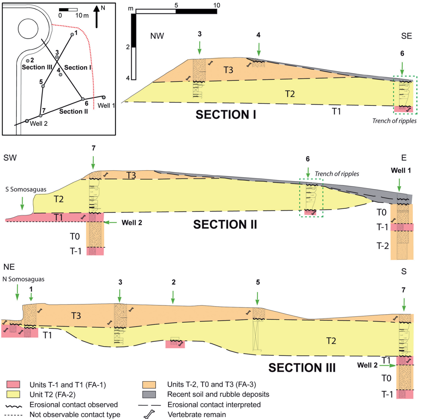
Figure 3. Reconstructed stratigraphic architecture along three cross-sections. Red dotted line indicates the lateral extent of the unit T2.
