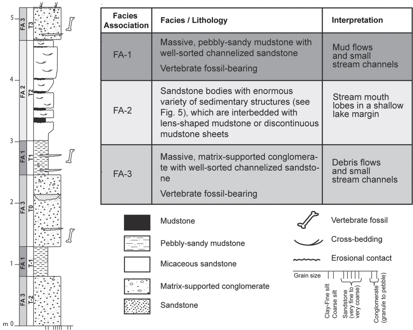
Figure 4. Synthetic stratigraphic log, stratigraphic units and general characteristics and interpretation of facies associations (FA-1, FA-2 and FA-3).
