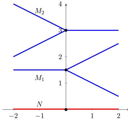
FIGURE 1. Projection \pi : M := M_1 \cup M_2 \rightarrow N
