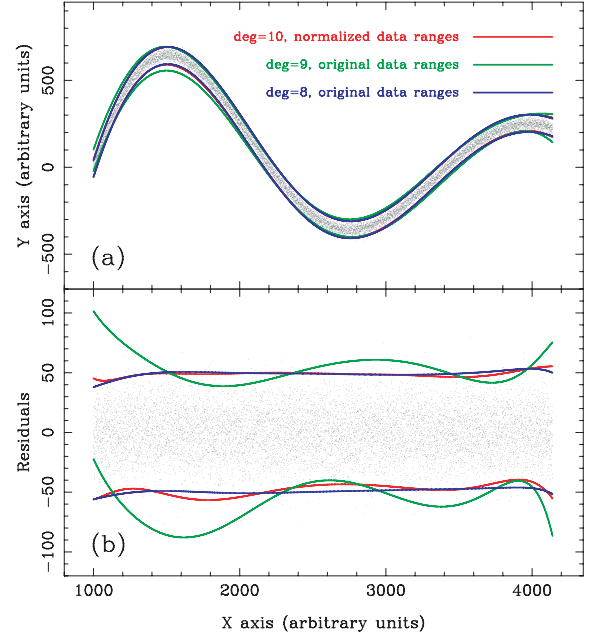
Figure B2. Example of the appearance of numerical errors in the boundary fitting with simple polynomials. The fitted data set consists in 10 000 points randomly drawn from the function y = \sin(1.5x)/(1+x) for x \in [0, 2\pi] , assuming a Gaussian error \sigma = 0.02 in the y-axis, and where prior to the data fitting the (x, y) coordinates were transformed using x_{\text{fit}} = 1000 + 500x_{\text{original}} and y_{\text{fit}} = 1000y_{\text{original}} in order to artificially enlarge the data ranges. Panel (a): bootstrapped data and fitted boundaries. Panel (b): residuals relative to the original sinusoidal function. In both panels the lines indicate the resulting fits for different polynomial degrees and normalization strategies (in all the cases \xi = 1000 , \alpha = 2 and \beta = 0 were employed). The continuous red lines are the boundaries obtained using polynomials of degree 10 and normalizing the data ranges prior to the fitting procedure. The green and blue lines correspond to the fits obtained by fitting polynomials of degrees 9 and 8, respectively, without normalizing the data ranges. Using the original data ranges the boundary fits start to depart from the expected location due to numerical errors for polynomials of degree 9. However, polynomials of degree 10 are still an option when the data ranges are previously normalized.
