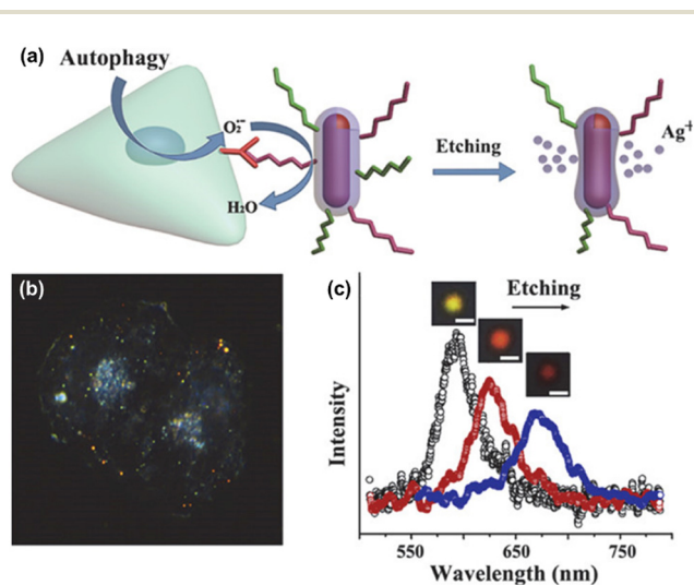
Fig. 10 (a) Illustration of the autophagy process of a cell producing superoxide radicals that etch the metal core-shell nanosensor. (b) Representative dark-field spectroscopy images of a HeLa cell studied by a relay of probes during the long autophagy process. (c) Scattering spectra of a single nanorod etched by superoxide radicals for 0, 30, and 60 minutes. Insets show dark-field scattering images of the probe in each status. Scale bar: 500 nm. Reprinted with permission from ref. 88. Copyright 2015 American Chemical Society.
