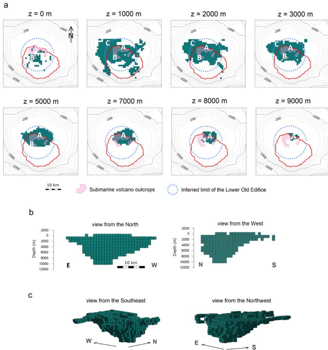
Figure 9. Magnetic model obtained by nonlinear inversion for a magnetization J = 1.5 \text{ A/m} , which can be considered a good representation of the main magnetic source beneath La Gomera, assuming that this source is a uniformly magnetized body. (a) Horizontal sections at different depths below sea level ( z ) of the described magnetic model. The contours show the bathymetry around the island, based on ETOPO1 data. The island's coastline is shown in red. The locations of the submarine volcano outcrops (Figure 1(c)) are superimposed to analyze possible correlations. The rough limits inferred by Ancochea et al. (2006) for the old shield basaltic volcano (Lower Old Edifice) are also indicated. Labels A–C identify the high magnetization areas in Figure 6. (b) Vertical views of the model from the north and from the west. (c) Three-dimensional perspective views of the model from the southeast and from the northwest.
