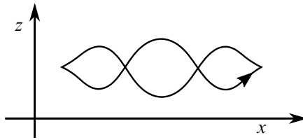
Figure 8: The basepoint (a horizontal knot) of the area twist loop in the front Geiges projection.
