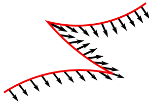
Figure 37: Deformation in the moduli space.
