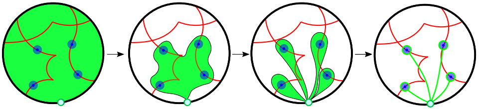
Figure 21: Homotopy between \gamma^\theta and the concatenation of n area twist loops for the case n = 4 represented in \mathbb{D}_G . We have drawn the zeros of the area function in blue. The concatenation of 4 area twist loops is represented by the green curve in the last step.
