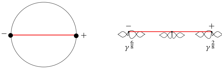
Figure 17: Geiges projection of the standard capping disk through horizontal immersions of the area twist loop. Left: capping disk in \text{LegImm}(\mathbb{R}^3) . Right: curve of strict Legendrian immersions in the front Geiges projection.
