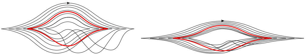
Figure 3: C^1 -approximation of the knot to the core, shown in the front projection. Left: front projection of the knot and the core (in red). Right: knot C^1 -close to the core.
