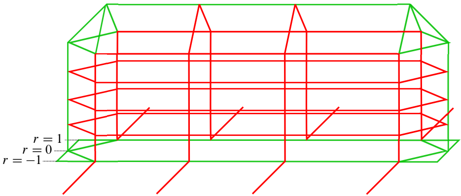
Figure 39: Construction of \tilde{\mathbb{D}} .
