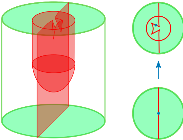
Figure 40: Schematic description of Lemma 8.2.1. The blue point in the middle of the circle represents \beta and the red middle circle in the cylinder the self-intersection (with nonzero area) created in the DS.
