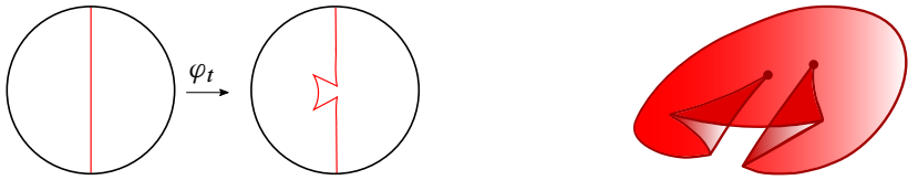
Figure 34: The 1–parameter family of disks \varphi_t: \mathbb{D} \rightarrow \mathcal{L}eg\mathcal{I}mm(\mathbb{R}^3) for t \in [0, 1] , described in Lemma 8.1.19. Left: Change in the topology of the disk in the moduli space via \varphi_t . Right: Birth of four cusps in the moduli space.
