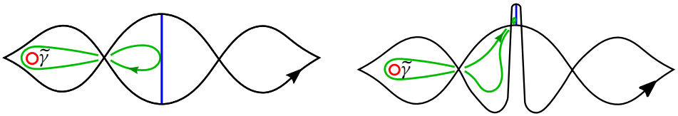
Figure 12: Cases where the three conditions are fulfilled: on the left, the tangent is -\partial_z , on the right, the tangent is \partial_z .
