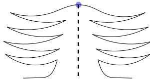
Figure 30: Legendrian finger construction process. The key tool is to create a huge tower of double stabilizations.
