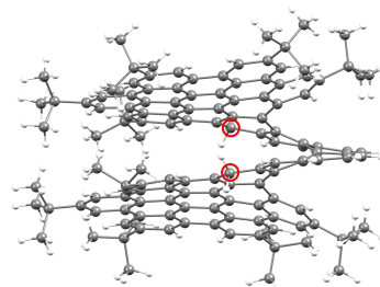
Figure 2. The core of \text{C}_{138}\text{H}_{122}^{3-} in 2 and 3 , ball-and-stick model.
