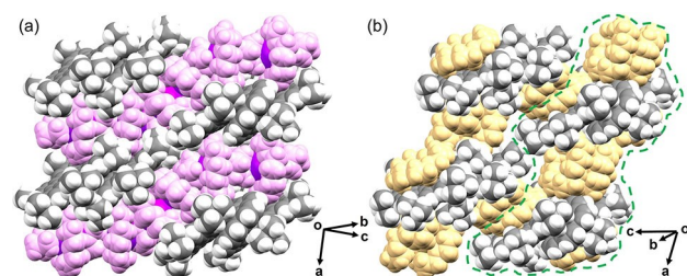
Figure 6. Solid-state packing in a) 2 and b) 3 , space-filling models. \{K^+(18\text{-crown-6})(THF)_n\} moieties are shown in purple, and \{Rb^+(18\text{-crown-6})_n\} moieties are shown in yellow.
