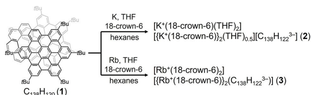
Scheme 1. Chemical reduction of 1 with K and Rb metals.
