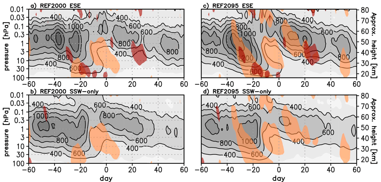
Fig. 7. Composite amplitude of planetary wavenumber-1 of geopotential height (m) at 50^\circ – 70^\circ\text{N} for a) ESEs and b) SSW-only events in the REF2000 simulation and c) ESEs and d) SSW-only events in the REF2095 simulation. Orange shading denotes where values for ESEs are statistically significantly different from those for SSW-only events at a 95% confidence level (Student's t-test). Red shading denotes where REF2095 composites are different from REF2000 composites at a 95% confidence level (Student's t-test).
