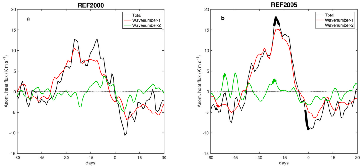
Fig. 6. Composite daily heat flux anomaly [ \text{K m/s} ] averaged between 45^\circ and 75^\circ\text{N} at 100 hPa from 60 days before to 30 days after the central date of the ESEs in the (a) REF2000 simulation and (b) REF2095 simulation. Black line: total anomalous flux, red line: wavenumber-1 component, and green line: wavenumber-2 component. Thick lines indicate where the REF2095 values are statistically different from the REF2000 values at a 95% confidence level (Student's t-test).
