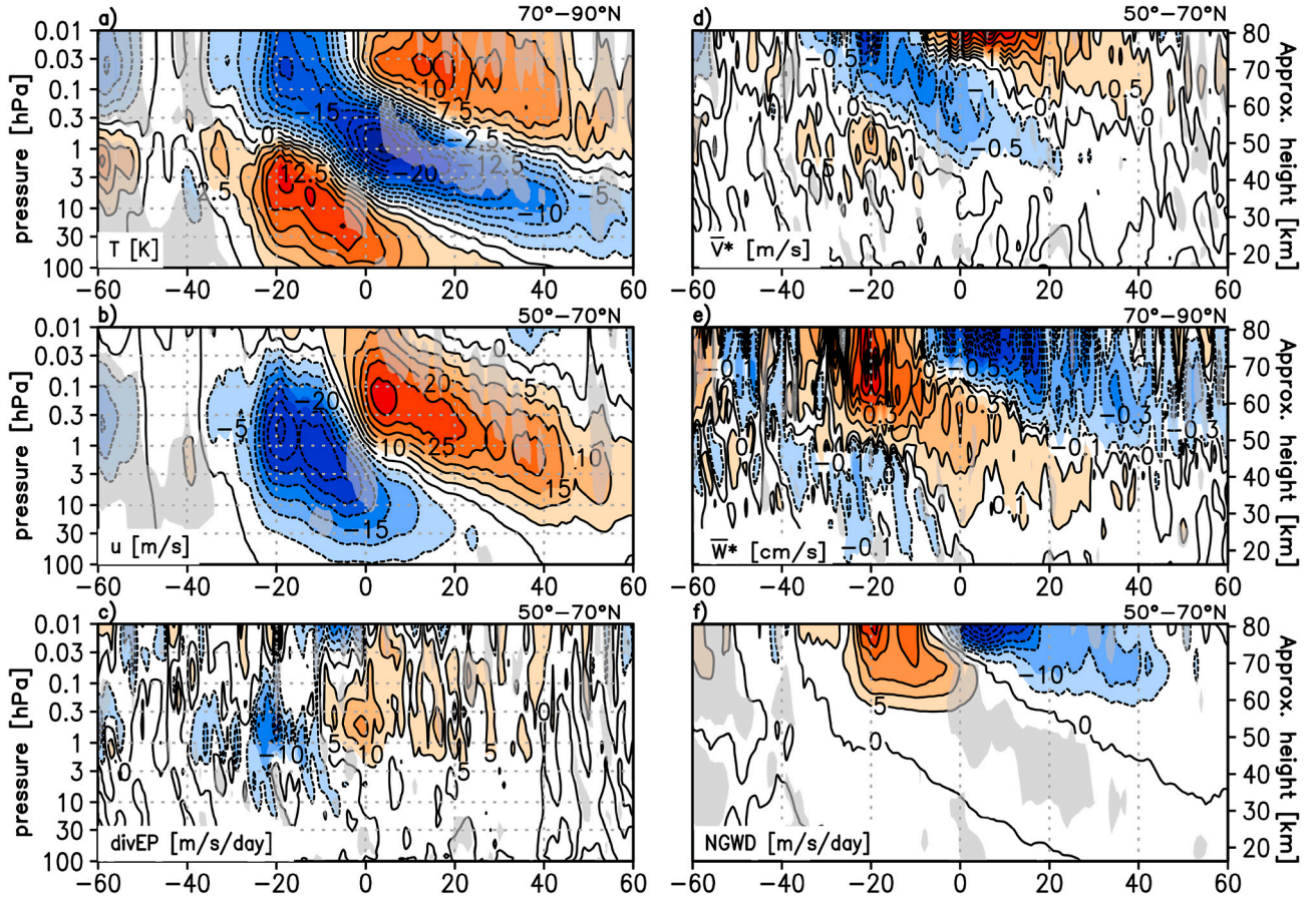
Fig. 3. As Fig. 1 but for the anomalies from the daily climatology of the fields. Gray shading shows where the anomalous ESE composite in the REF2000 simulation is significantly different (at a 95% confidence level) from the anomalous ESE composite in the REF2095 simulation (compare with Fig. 9) according to Student's t-test.
