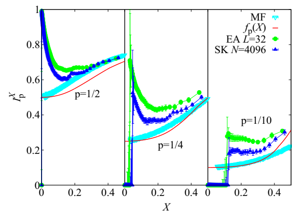
FIG. 6. (Color online) We compare the self-consistent approximation of Eq. (11), f_p(X) , to the data obtained for the largest lattice sizes both for the EAI and the SK models. We also include the mean-field prediction, as constructed from a weight-generation method (see text and [51]). We show on the left p = \frac{1}{2} (i.e., the median), in the center p = \frac{1}{4} , and on the right p = \frac{1}{10} .
