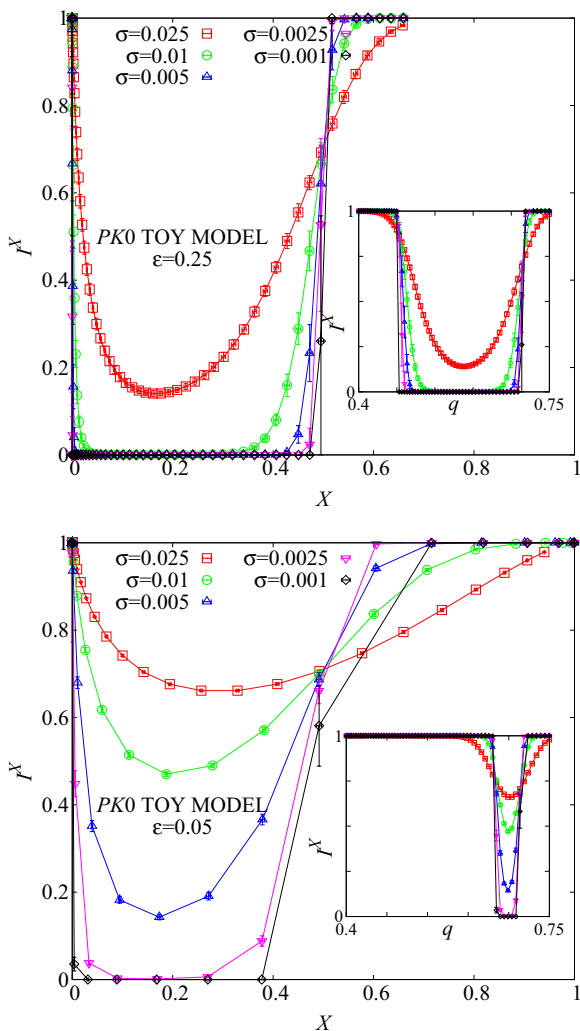
FIG. 7. (Color online) PK0 toy model: f \equiv I(q)^X(q) as a function of X(q) (main plots) and as a function of q (insets). q_{J_0} = 0.7 . Top: The width of the distribution of the position of the peak is \epsilon = 0.25 . Bottom: \epsilon = 0.05 .
