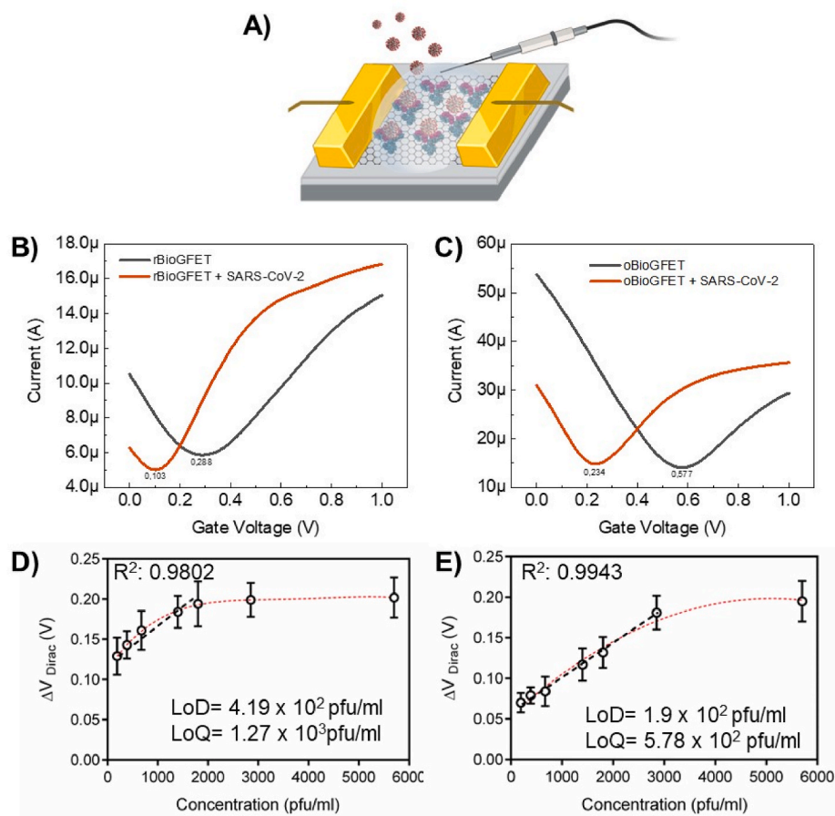
Fig. 5. (A) Schematic diagram of the aqueous-solution-gated GFET in antibody-conjugated graphene incubated with SARS-CoV-2. Representative I_{DS}-V_{GS} output curves of (B) random and (C) oriented functionalized sensors before and after incubation with SARS-CoV-2 (5800 pfu/ml) for 1 h. Dose-dependent response curve in the detection of SARS-CoV-2 virus in VTM solutions: (D) Random BioGFET; (E) Oriented BioGFET. Red dotted line: trend curve. Black long dashed line: linearity range. The error bars for (D) and (E) were calculated using data from four different chips ( n = 4 ). The LoD and LoQ values were calculated using the ‘standard deviation of a linear response and a slope’ approach as described in ‘Validation of Analytical Procedures Q2 (R2)’ guidelines (published by the ICH and adopted by both EMA and FDA) (ICH Q2(R2) Validation of analytical procedures - Scientific guideline, 2022a; Q2(R2) Validation of Analytical Procedures, 2022) and as detailed in Materials and Methods.
