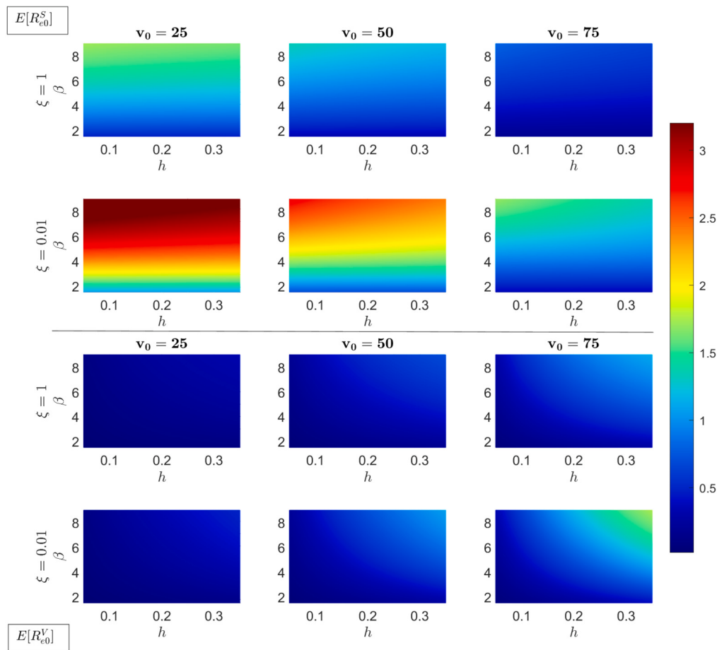
Fig. 5. E[R_{e0}^V] and E[R_{e0}^S] as a function of \beta and h , for different values of \xi and v_0 .
