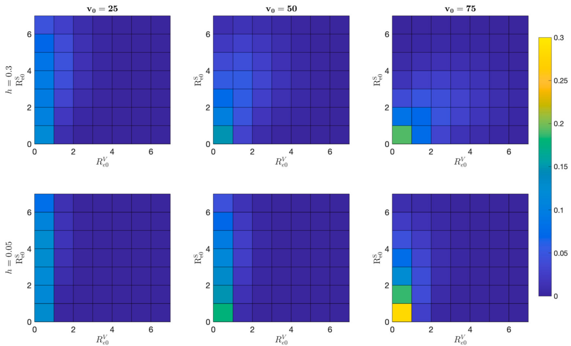
Fig. 4. Joint mass probability distribution function of (R_{e0}^V, R_{e0}^S) for h \in \{0.05, 0.3\} , v_0 \in \{25, 50, 75\} and initial state (v_0, N - v_0 - 1, 1) , when N = 101 , \beta = 9 , \xi = 0.01 and \gamma = 1 .
