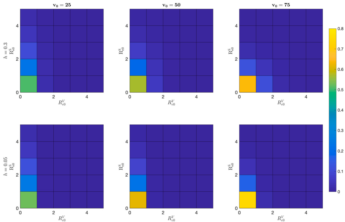
Fig. 3. Joint mass probability distribution function of (R_{e0}^V, R_{e0}^S) for h \in \{0.05, 0.3\} , v_0 \in \{25, 50, 75\} and initial state (v_0, N - v_0 - 1, 1) , when N = 101 , \beta = 1.2 , \xi = 0.01 and \gamma = 1 .
