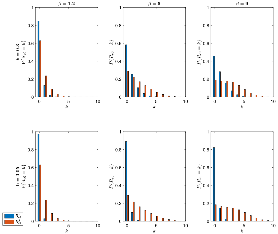
Fig. 2. R_{e0}^V and R_{e0}^S marginal probability mass functions for \beta \in \{1.2, 5, 9\} and h \in \{0.05, 0.3\} , when N = 101 , \xi = 0.01 , \gamma = 1 and for initial state (50, 50, 1) .
