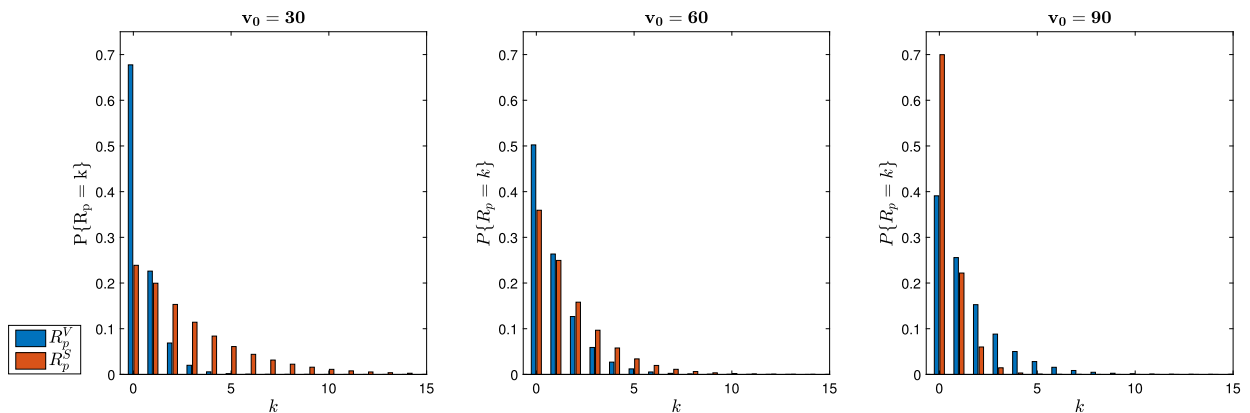
Fig. 10. Influenza in a boarding school. R_p^V and R_p^S marginal probability mass functions for R_0 = 3.652 , \xi = 0.01 and h = 0.3821 , when N = 101 and for v_0 \in \{30, 60, 90\} .
