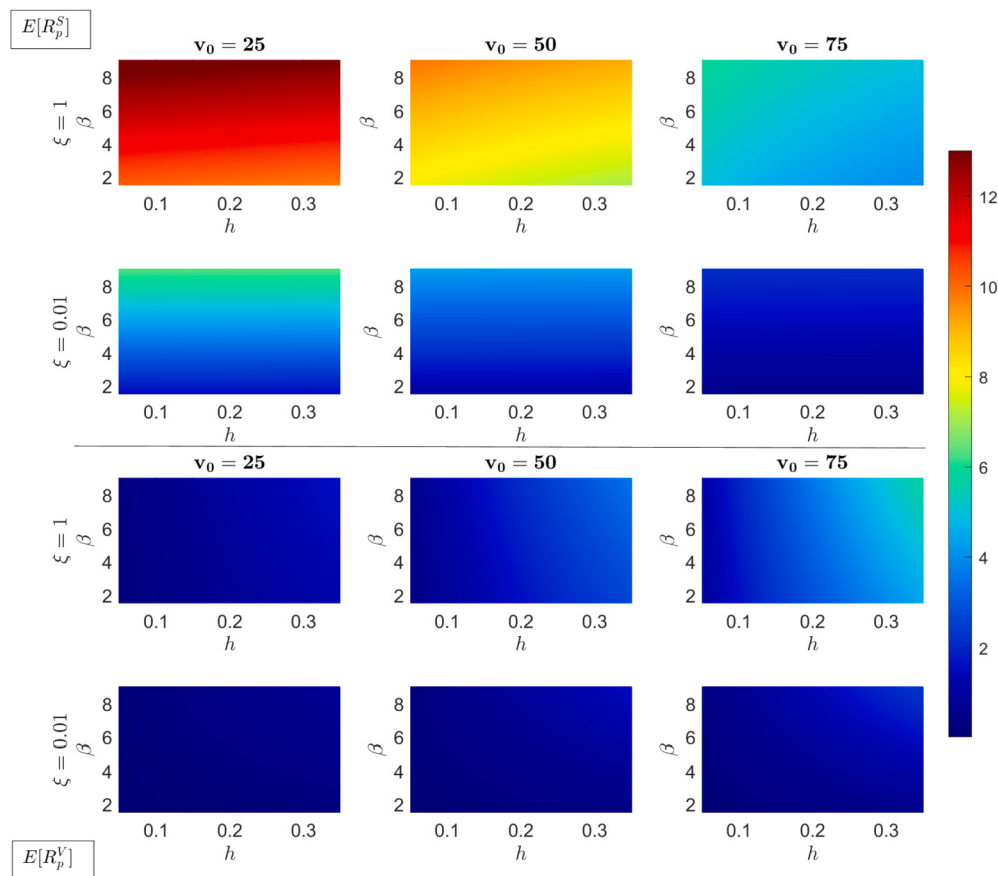
Fig. 8. E[R_p^S] and E[R_p^V] as a function of \beta and h . Different scenarios arise in a population of N = 101 individuals, with an initial infectious individual and \gamma = 1 when v_0 \in \{25, 50, 75\} and \xi \in \{0.01, 1\} .
