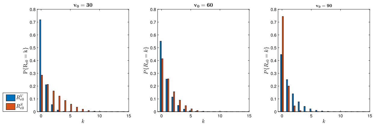
Fig. 9. Influenza in a boarding school. R_{e0}^V and R_{e0}^S marginal probability mass functions for R_0 = 3.652 , \xi = 0.01 and h = 0.3821 , when N = 101 and for v_0 \in \{30, 60, 90\} .
