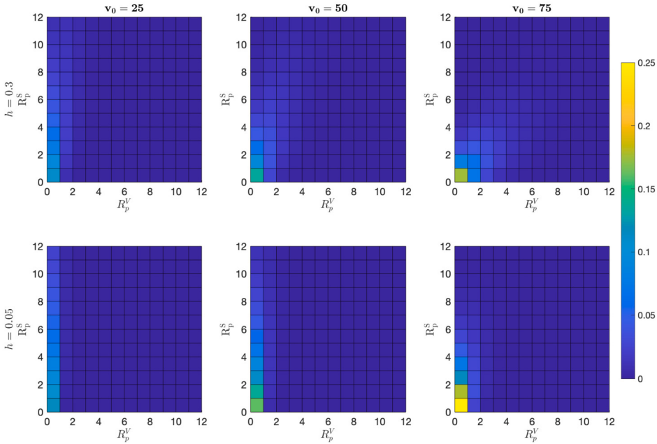
Fig. 7. Joint probability mass distribution function of (R_p^V, R_p^S) for several values of h and vaccination levels ( v_0 ) in a population of N = 101 individuals, with an initial infective individual and \beta = 9 , \gamma = 1 and \xi = 0.01 .
