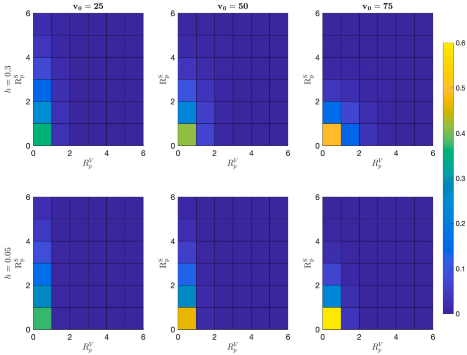
Fig. 6. Joint probability mass distribution function of (R_p^V, R_p^S) for several values of h and vaccination levels ( v_0 ) in a population of N = 101 individuals, with an initial infective individual, \beta = 1.2 , \gamma = 1 and \xi = 0.01 .
