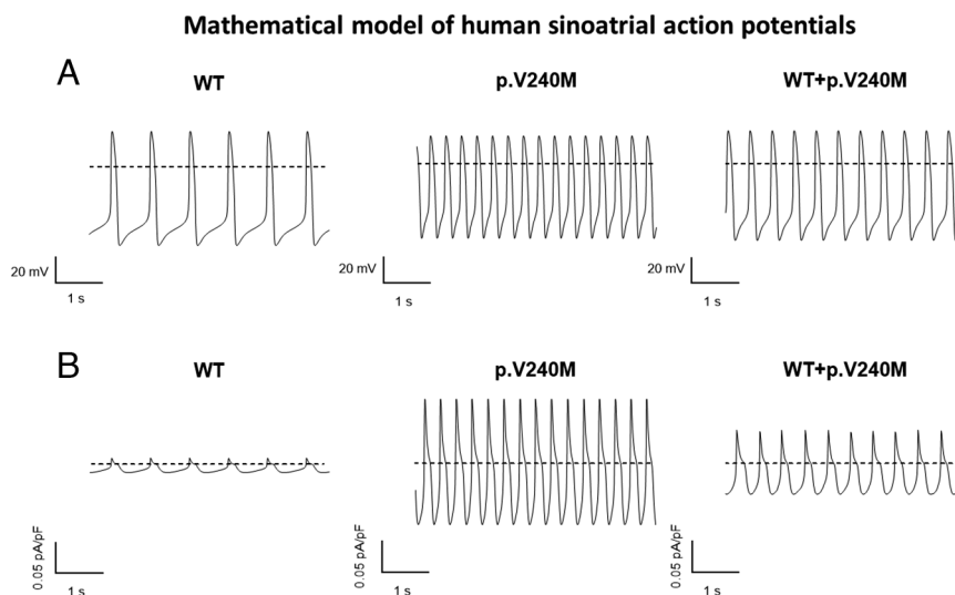
Fig. 7. Mathematical model of human sinoatrial node cell action potential. (A and B) APs (A) and I_f (B) obtained when running the model under basal conditions (WT; Left), or after introducing the experimentally measured I_{\text{HCN4}} changes induced by p.V240M alone (center) or together with WT (Right). The dotted lines represent the zero membrane potential (A) and current (B) levels.
