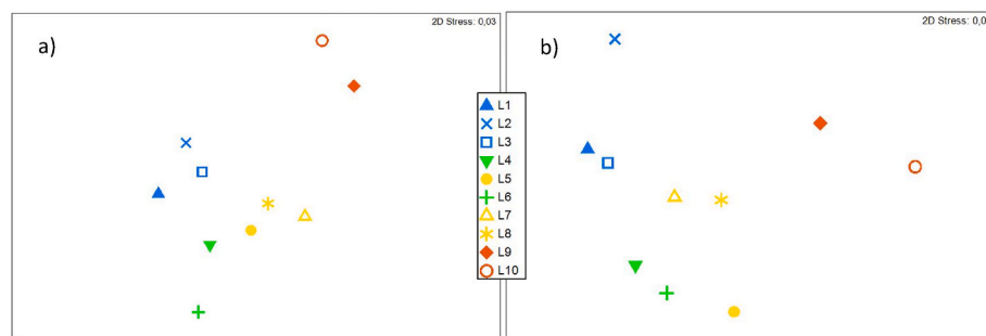
Fig. 5. Non-metric multidimensional scaling (nMDS) diagrams (Anderson et al., 2008) of the 10 locations (L1: Malpica; L2: Cedeira; L3: Luarca; L4: Lastres; L5: San Vicente; L6: Somocuevas; L7: Kobaron; L8: Ea; L9: La Herradura; and L10: Cabo Palos) based on square-root transformed abundances and Bray-Curtis similarities. a) observed pattern. b) modelled pattern. Colours are based on 43% similarity clustering (Fig. 2b).
