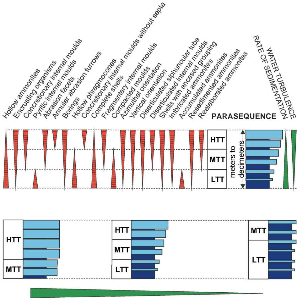
Fig. 4.-Frequency of different taphonomic characters displayed by ammonites included in a shallowing-upwards sequence or parasequence in carbonate outer platform, forming a positive taphosequence and different taphorecords. LTT = low turbulence taphorecord. MTT = moderate turbulence taphorecord. HTT = high turbulence taphorecord.
