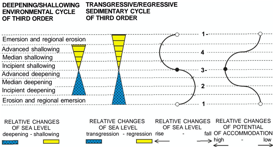
Fig. 6.- Relative changes of the potential of accommodation (i.e., subsidence and eustasy) and relative changes of sea level, two fundamental concepts of sequence stratigraphy, have conditioned the development of transgressive/regressive sedimentary cycles and environmental cycles of deepening/shallowing in carbonate epicontinental platforms. The curve representing relative changes of sea level during the development of transgressive/regressive sedimentary cycles of third order may be subdivided into four parts to differentiate four successive phases: 1) rapid fall, 2) increasing rate of rise, 3) rapid rise, 4) decreasing rate of rise. From the phase of incipient deepening until that of advanced shallowing, six successive phases can be distinguished in an environmental cycle of deepening/shallowing.
