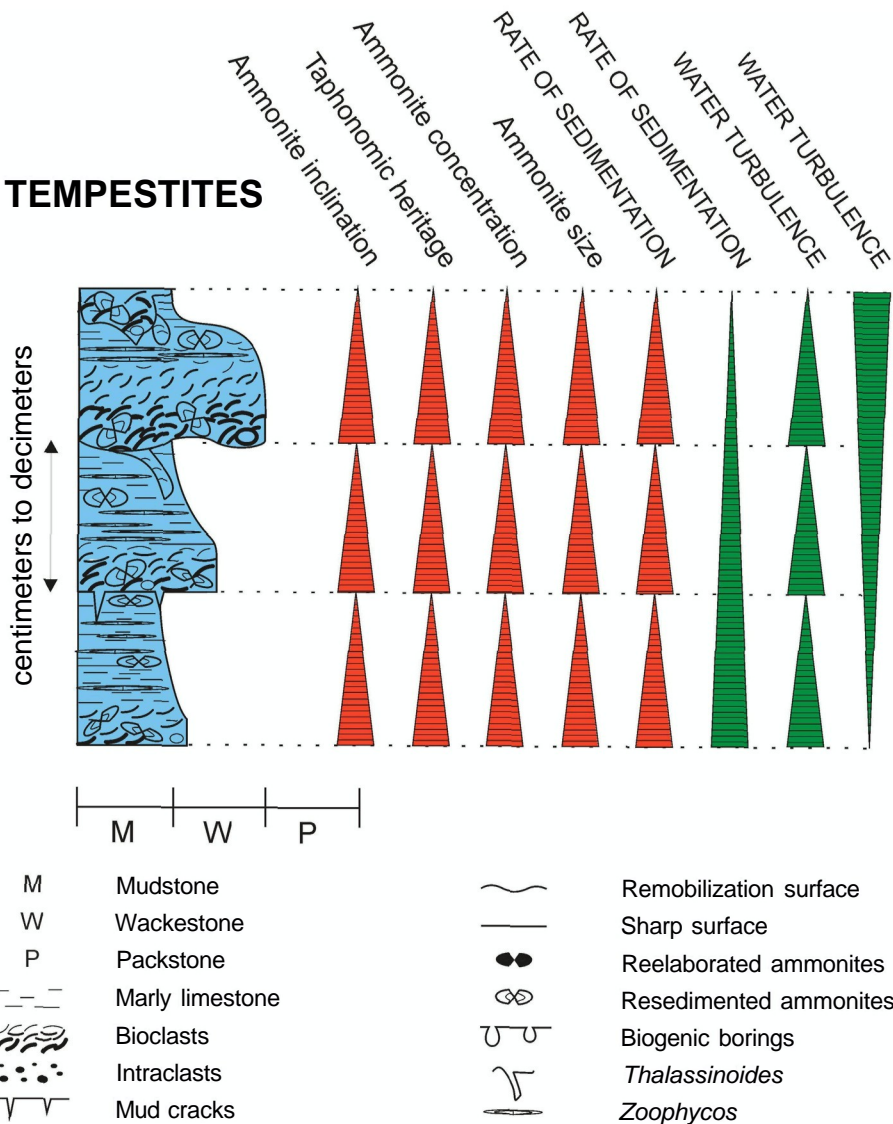
Fig. 3.-Frequency of different taphonomic characters displayed by ammonites included in tempestites of carbonate outer platform. During the development of a tempestite, in carbonate outer platform environments, the water turbulence and the rate of sedimentation decrease. During the development of such tempestites, consequently, the ammonite size, the ammonite concentration, the taphonomic heritage and the ammonite inclination decrease.
