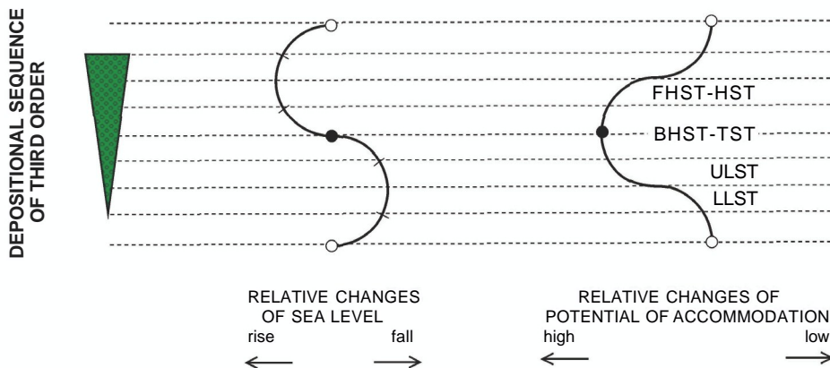
Fig. 5.- Different depositional systems and successive phases which can be distinguished during the development of a depositional sequence of third order. LLST = lower lowstand systems tract. ULST = upper lowstand systems tract. BHST or TST = backstepping highstand (or transgressive) systems tract. FHST or HST = forestepping highstand systems tract.
