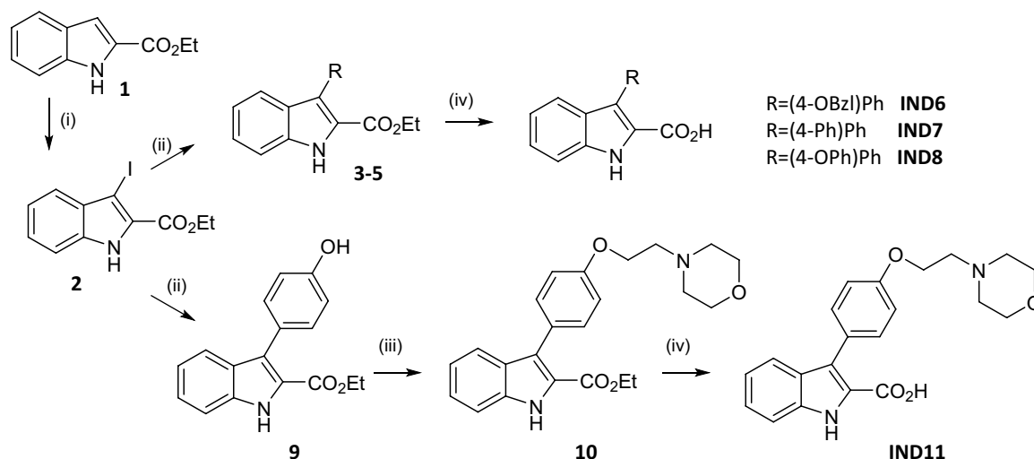
Scheme 1. (i) iodosuccinimide, DMF, 0 °C, 1 h; (ii) toluene:ethanol:water:1,4-dioxane (1:3:6:10), R-B(OH) 2 , Pd (PPh 3 ) 4 , K 2 CO 3 , 85 °C, 18 h; (iii) K 2 CO 3 , EtOH, 85 °C, 18 h (iv) KOH, EtOH, 100 °C, 18 h.
