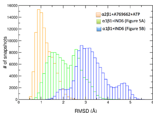
Figure 6. Distribution of the positional deviation (RMSD; Å) of the backbone atoms that shape the ATP-binding along the trajectories run for the two binding modes of IND6 bound to AMPKα1β1 (shown in Fig. 5A,B), and for the ternary complex between A-769662, ATP and AMPKα2β1 (data taken from 24 ).
