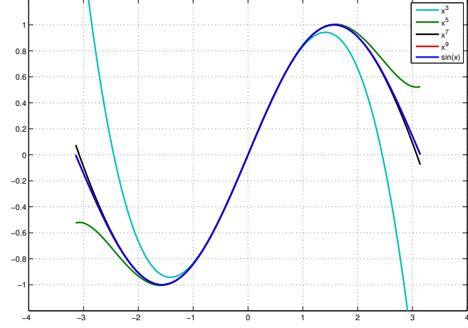
(b) \sin(x) , polinomios 3, 5, 7 y 9 grados (b) polynomials 3, 5, 7 and 9 degrees
