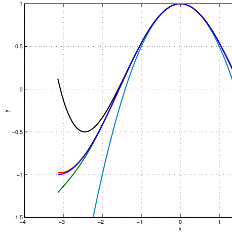
(a) \cos(x) , polinomios 2, 4, 6 y 8 grados (a) polynomials 2, 4, 6 and 8 degrees
