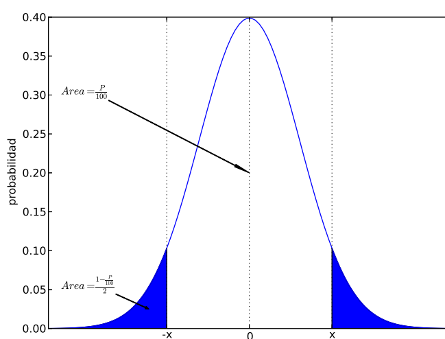
Figura 10.12: Intervalo de probabilidad P\% Figure 10.12: Probability interval P\%
