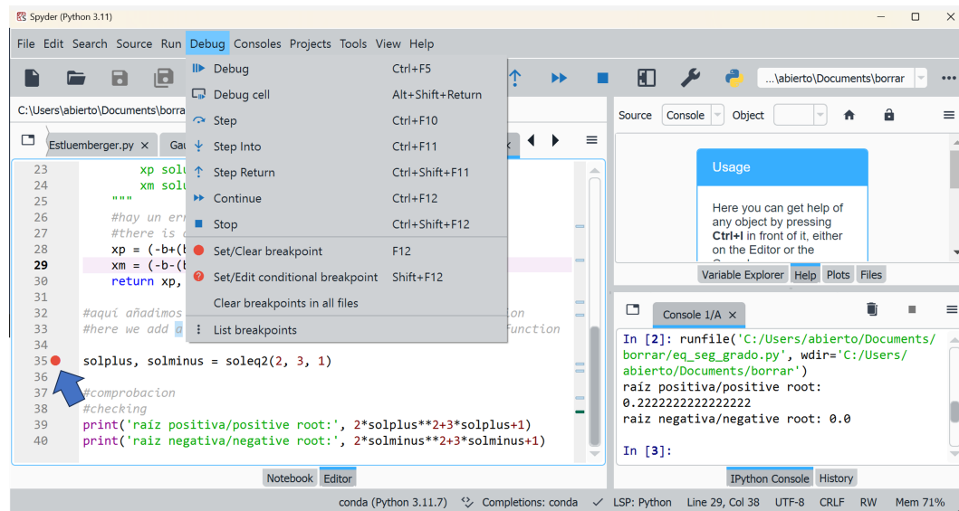
Figura 2.11: Breakpoint activo señalado con una flecha azul, y menú desplegable debug Figure 2.11: Active Breakpoint pointed by a blue arrow and debug drop-down menu
