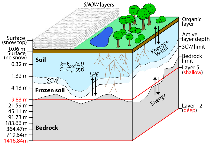
FIG. 1. Simplified vertical scheme of the JSBACH land surface model component in the northern high latitudes. The shallow (5-layer) and deep (12-layer) BBCP-depth configurations are marked in red. Soil depth (bedrock limit) varies in every model grid point as prescribed by the respective soil parameter dataset (SPD). Soil moisture is present above the bedrock only. The representation of snow (SNOW), dynamic soil thermal properties (DCC, with k = thermal conductivity and C = heat capacity), latent heat transfer (LHE), and supercooled water (SCW) are regulated by the given model configurations of hydro-thermodynamic soil coupling. See Fig. 1 in Part I for a comparison of the differences in model features considered herein.
