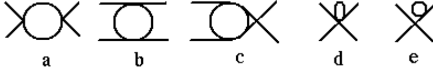
FIG. 1. Generic one-loop Feynman diagrams that have to be evaluated in meson-meson scattering.
