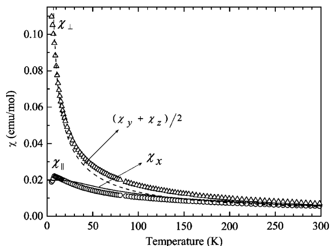
FIG. 7. Magnetic susceptibility per \text{Nd}^{3+} versus temperature for single-crystal \text{Nd}_2\text{BaCuO}_5 oxide. The triangles and circles correspond to the magnetic susceptibility per \text{Nd}^{3+} measured along the a and the c axis, respectively. The solid, and dashed lines correspond to the calculated magnetic susceptibilities per \text{Nd}^{3+} , \chi_x and (\chi_y + \chi_z)/2 , respectively.
