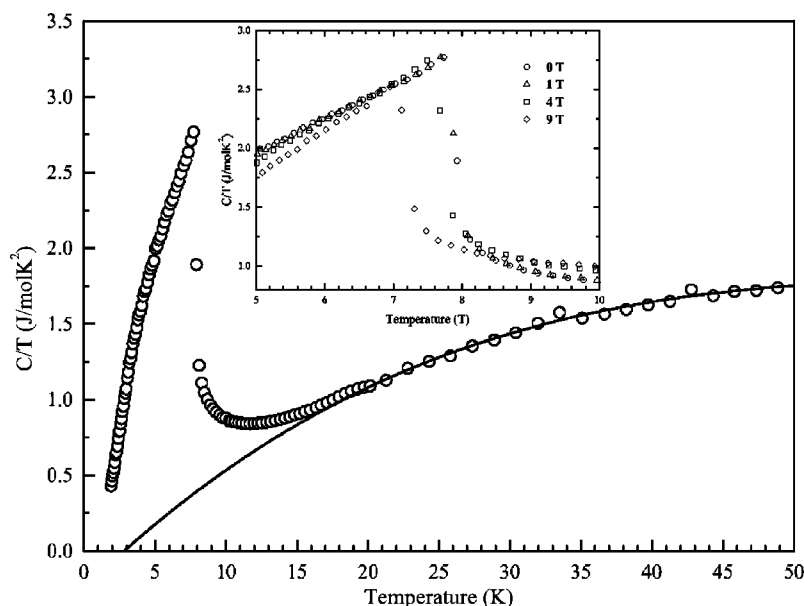
FIG. 5. Temperature dependence of the total specific heat measured at 0 T. The inset shows the variation of the total specific heat as a function of the temperature at different magnetic field strengths. The solid line represents the calculated electronic and lattice contributions to the total specific heat.
