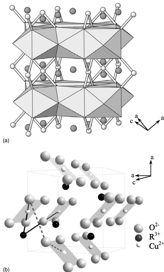
FIG. 1. Perspective views of \text{Nd}_2\text{BaPtO}_5 -type structure of the so-called brown phases \text{R}_2\text{BaCuO}_5 ( \text{R} : La or Nd), showing (a) the \text{RO}_8 layers (gray polyhedra), square-planar \text{CuO}_4 (stick and balls), and barium atoms (dark gray circles); and (b) the different magnetic interaction pathways as dashed and bold lines (see text).
