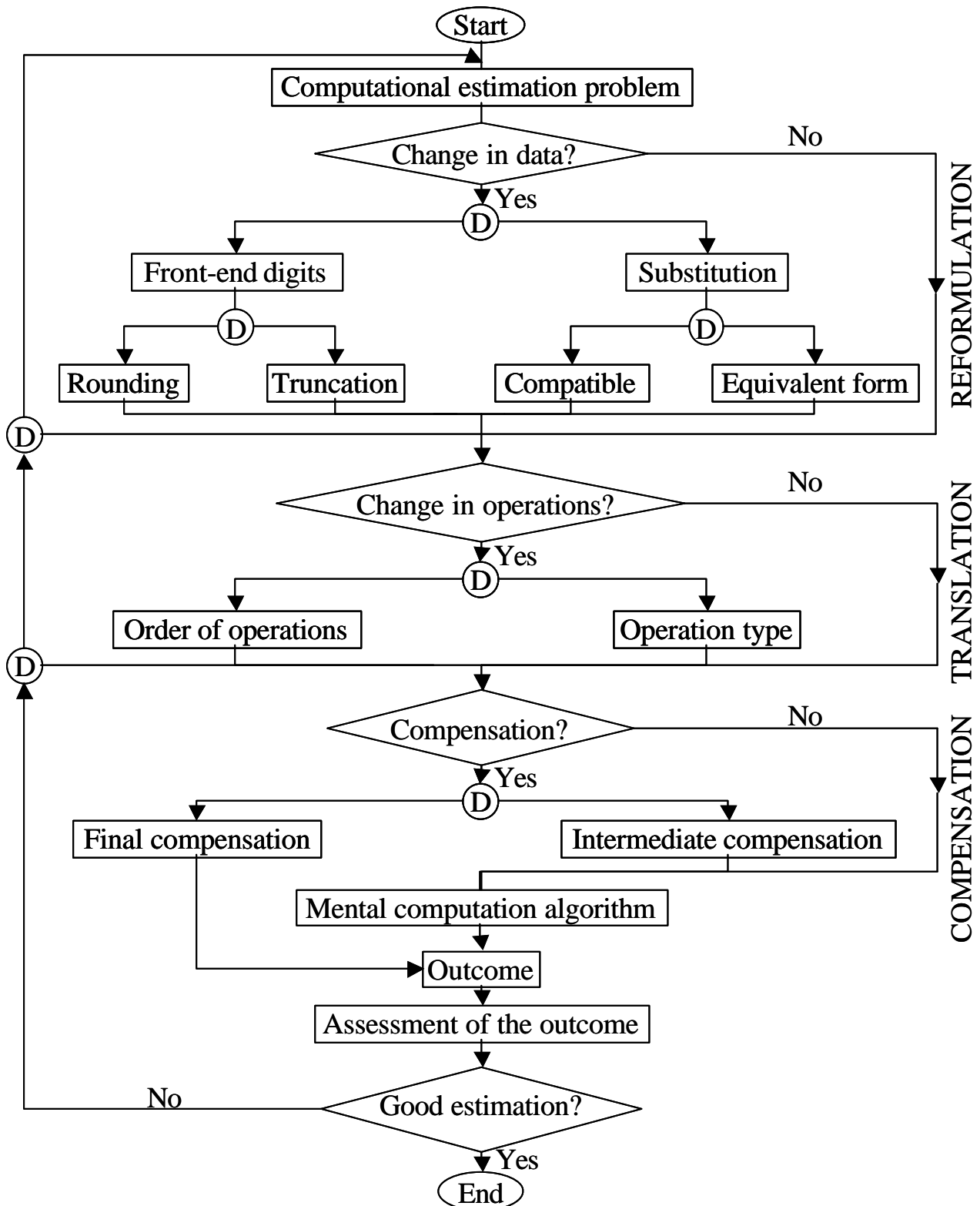
Figure 1. Graphic of computational estimation strategies. The symbol D represents the points of the procedure where one must to take a decision
