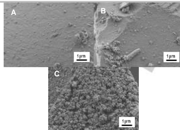
Figure 7. SEM images of non-soaked S3 (A), 72 hours soaked S3 with no APase (B), and 72 hours soaked S3 with APase (C).
