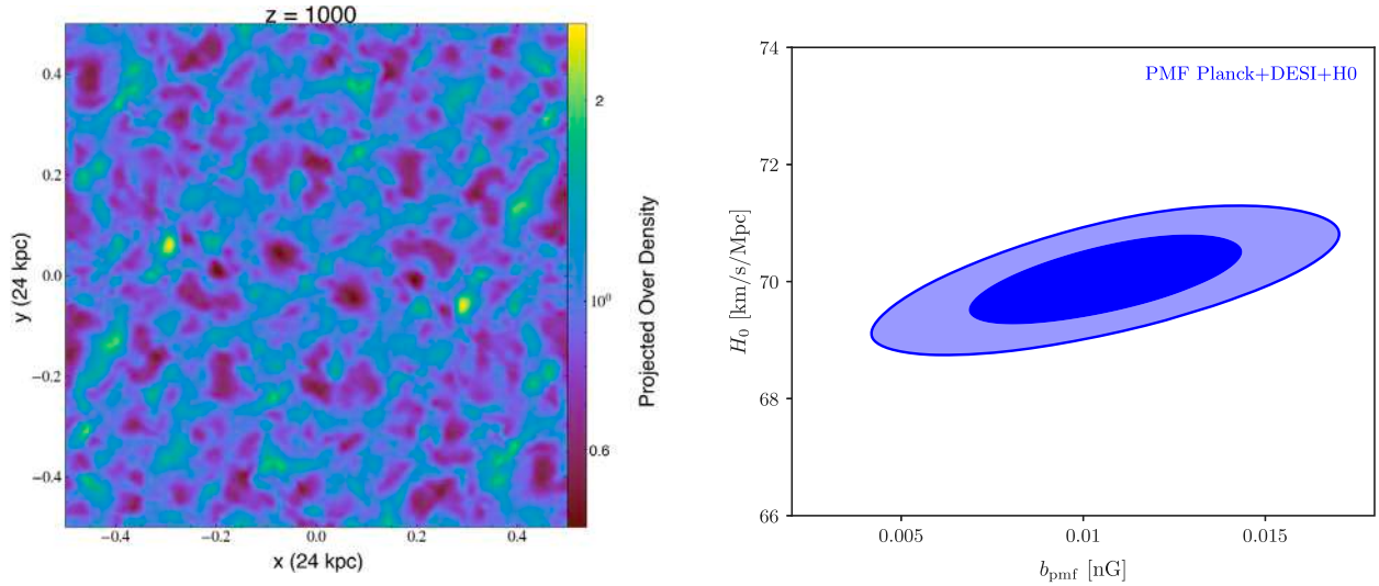
Fig. 78. Left: Results of an MHD simulation [3852] starting at redshift z = 4500 with an initial comoving magnetic field of 0.526 \text{ nG} with Batchelor spectrum and initially vanishing density perturbations and peculiar flows. The figure shows the (projected) density fluctuations generated at z = 1000 by the stochastic magnetic field. Right: Preliminary results of a MCMC comparing the theoretical prediction of a \Lambda\text{CDM} model with a PMF with Batchelor spectrum to the combination of Planck CMB data [192], DESI-1Y BAO data [699], and the SH0ES [34] Hubble constant determination. It is seen that a final magnetic field of B \approx 0.01 \text{ nG} is preferred leading to Hubble constants of H_0 \approx 70 \text{ km s}^{-1} \text{ Mpc}^{-1} , significantly larger than those predicted in \Lambda\text{CDM} without a PMF. This field strength is close to that needed to explain observed cluster magnetic fields entirely by a PMF.
