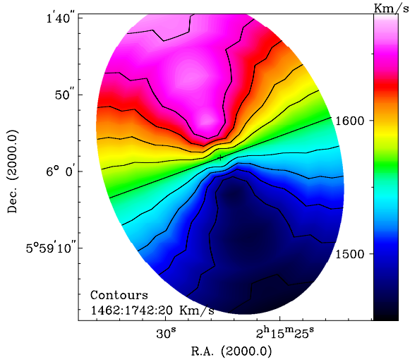
Figure 7. Model map derived from the rotation velocities previously obtained in the rotation curve.
