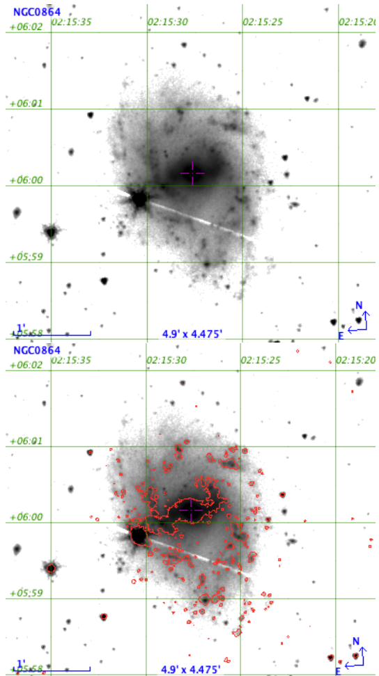
Figure 5. Top: 3.6 \mu m S^4G image. Bottom: the same with H\alpha contours at 1.1 \cdot 10^{36} erg/s, taken from the ACAM image.
