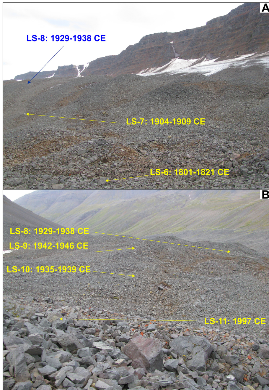
Fig. 10. The proto-rock glacier at the top of the active debris covered glacier, close to the current front of the Hóðinsdalsjökull glacier. A) Frontal area of the proto-rock glacier from the east in 2018. B) Root area of the proto-rock glacier viewed from the west. The location and dates (in CE years) of the LS are indicated in all panels.
