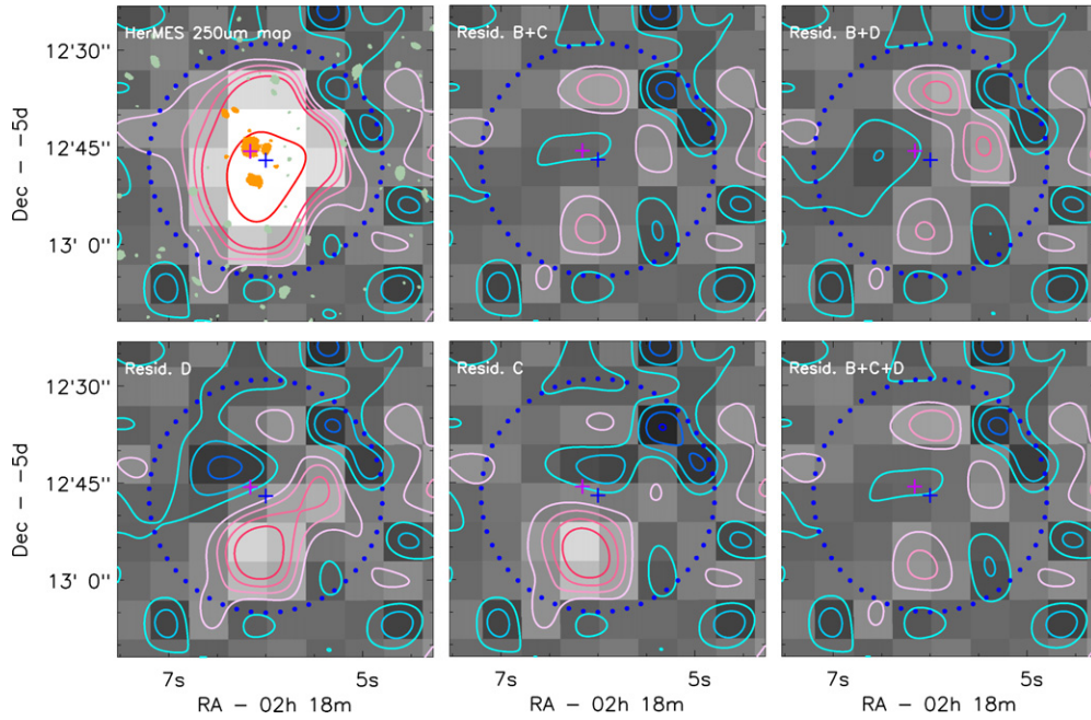
Figure 15. Demonstration of the decomposition in 250 \mu\text{m} for UDS01. The first panel shows the original 250 \mu\text{m} image, while the others show the residual maps of the different decomposition schemes where different input sources are considered (labeled on top). Legends are the same as in Figure 5. This is a degenerate case. While automatically iterative fit settles on B+C, the trial-and-error run using B+D still produces satisfactory results. However, the fit without the inclusion of B are not acceptable.
