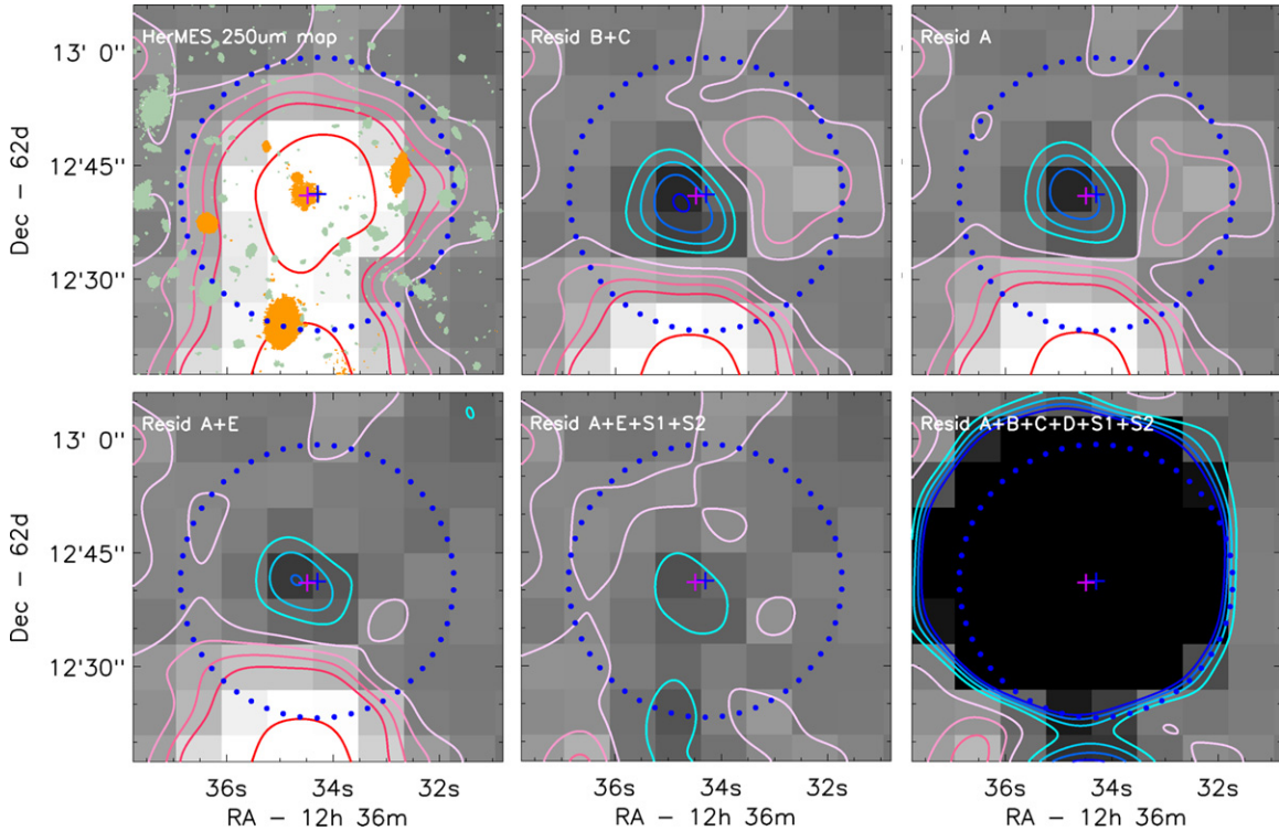
Figure 5. Demonstration of the decomposition in 250\ \mu\text{m} for GOODS-N06. The first panel shows the original 250\ \mu\text{m} image, while the others show the residual maps of the different decomposition schemes where different input sources are considered (labeled on top). The “B+C” panel is for the automatically interactive fit that fails to provide a satisfactory result, while the rest are for different trial-and-error runs where the input objects are interactively decided. The best result is produced by the “A+E+S1+S2” scheme (see text). All images are displayed in positive, i.e., using white for the positive values and black for the negative values. The contours coded in “warm” and “cold” colors indicate the different positive (i.e., residuals) and negative (i.e., over-subtraction) levels, respectively: the positive level increases from light pink to dark red, and the negative level increases from light green to deep blue. The contour starts at the level of \pm 0.4\ \text{mJy pixel}^{-1} , and increases or decreases at a step size of 0.4\ \text{mJy pixel}^{-1} . In the first panel which shows the original 250\ \mu\text{m} image, the H_{160} -band objects are superposed as the gray-green segmentation maps, among which the candidate counterparts are further highlighted in orange. In all panels, the blue dotted circle is 18'' in radius. The blue and the magenta crosses mark the 250\ \mu\text{m} source centroid and the VLA 1.4 GHz source position, respectively.
