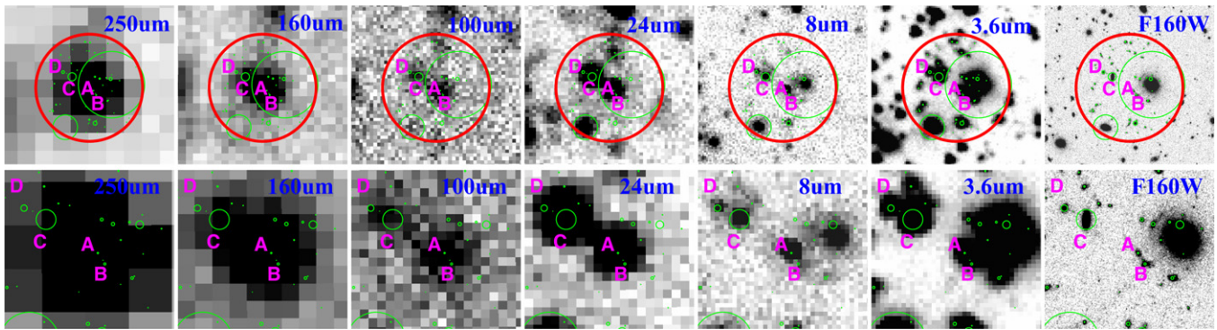
Figure 7. FIR to near-IR images of GOODS63. The organization and the legends are the same as in Figure 2. This source does not have MIPS 70\mu\text{m} data. The possible contributors to the 250 \mu\text{m} emission are labeled by the letters in purple.
