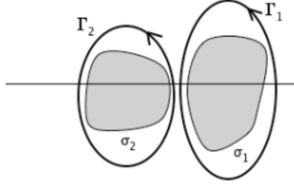
Figure 3.2: \sigma(F) = \sigma_1 \cup \sigma_2 .
