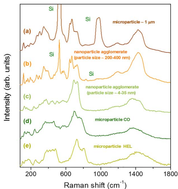
Figure 5. Raman spectra from synthetic \epsilon -Fe 2 O 3 . Comparison between different Raman spectra collected from different samples which contain \epsilon -Fe 2 O 3 : (a) single microparticle [López-Sánchez et al. , 2016a], (b) microagglomerate of nanoparticles [López-Sánchez et al. , 2016a], (c) nanoparticle agglomerate [López-Sánchez et al. , 2016b], (d) microparticle collected from CO (Figure 3c), and (e) microparticle acquired from HEL (Figure 4c).
