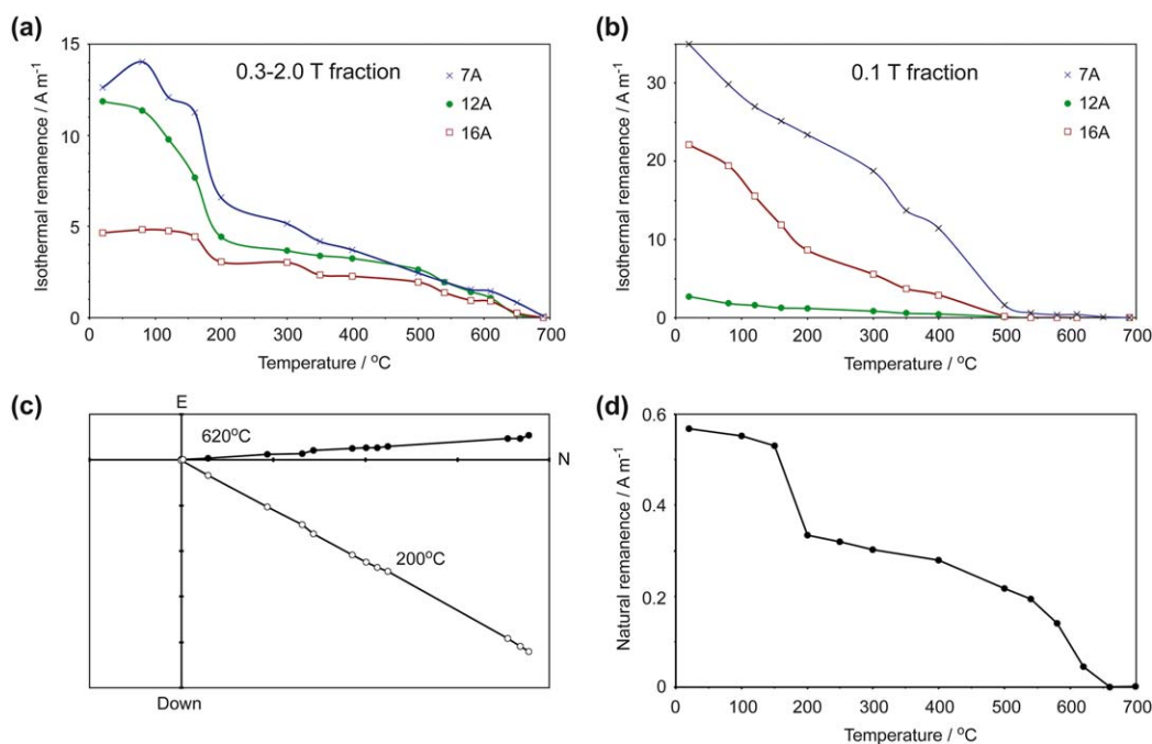
Figure 2. Representative thermal demagnetization of orthogonal isothermal and natural remanences from different CO samples (7A, 12A, and 16A). (top) Stepwise thermal demagnetization of two orthogonal IRMs in CO samples (a) intensity decay of the high coercivity (the 0.3-2 T) IRM fraction, showing the HCSLT phase. (b) Intensity decay of the low coercivity (0.1 T) magnetic component. (bottom) Thermal demagnetization of the Natural remanent magnetization of a representative sample from CO: (c) Zijderveld diagram and (d) intensity decay. In Figure 2c, closed and open symbols represent projection in the horizontal and vertical planes, respectively. Initial NRM of sample displayed in Figure 2c is 1.35 A/m.
