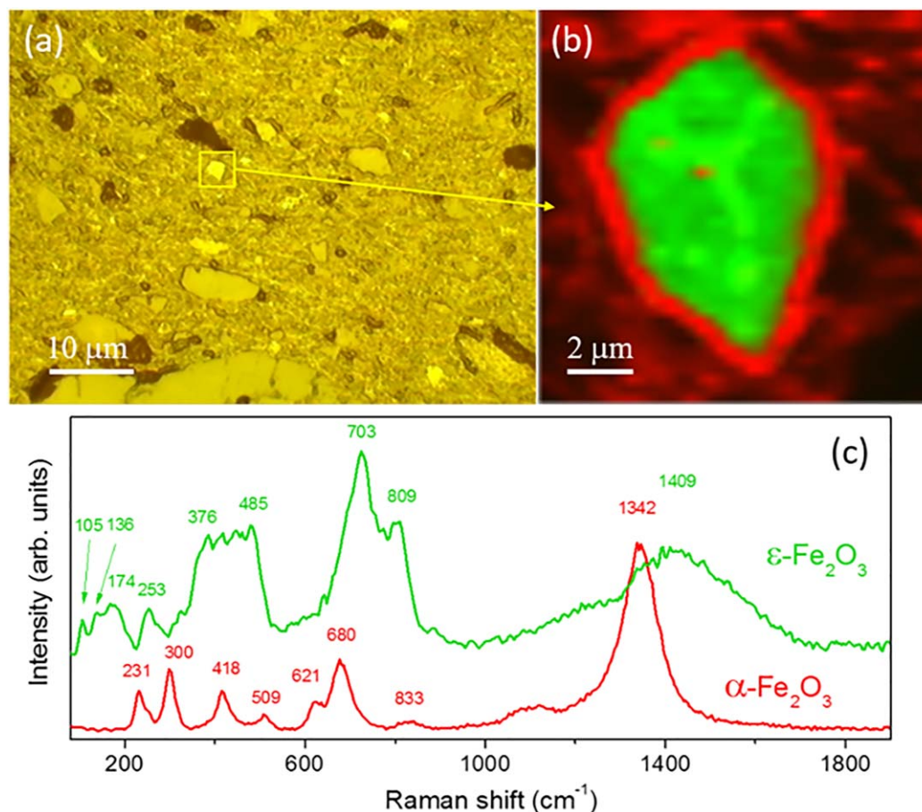
Figure 4. (a) Optical image of sample HEL. (b) In-plane Raman intensity image obtained from mapping the region marked with a yellow square in Figure 4a. (c) Average Raman spectra obtained from in-plane Raman image. See Figure 3 caption for spectra measurement and calculation details.
