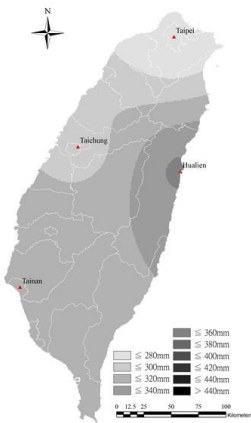
Figure 1 10-year return level
