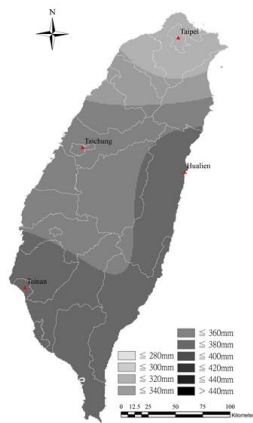
Figure 2 20-year return level
