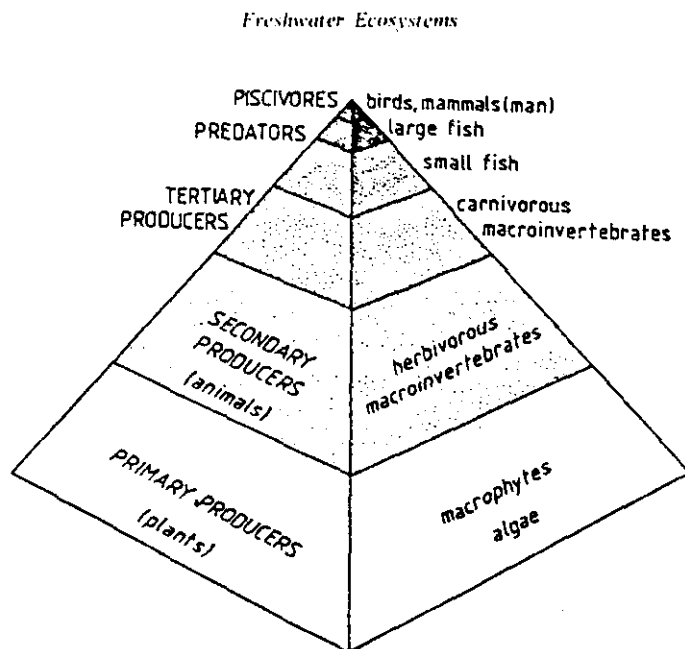
Diagram of a 'trophic pyramid' indicating the relative biomass at each trophic level and the potential for bioaccumulation.
