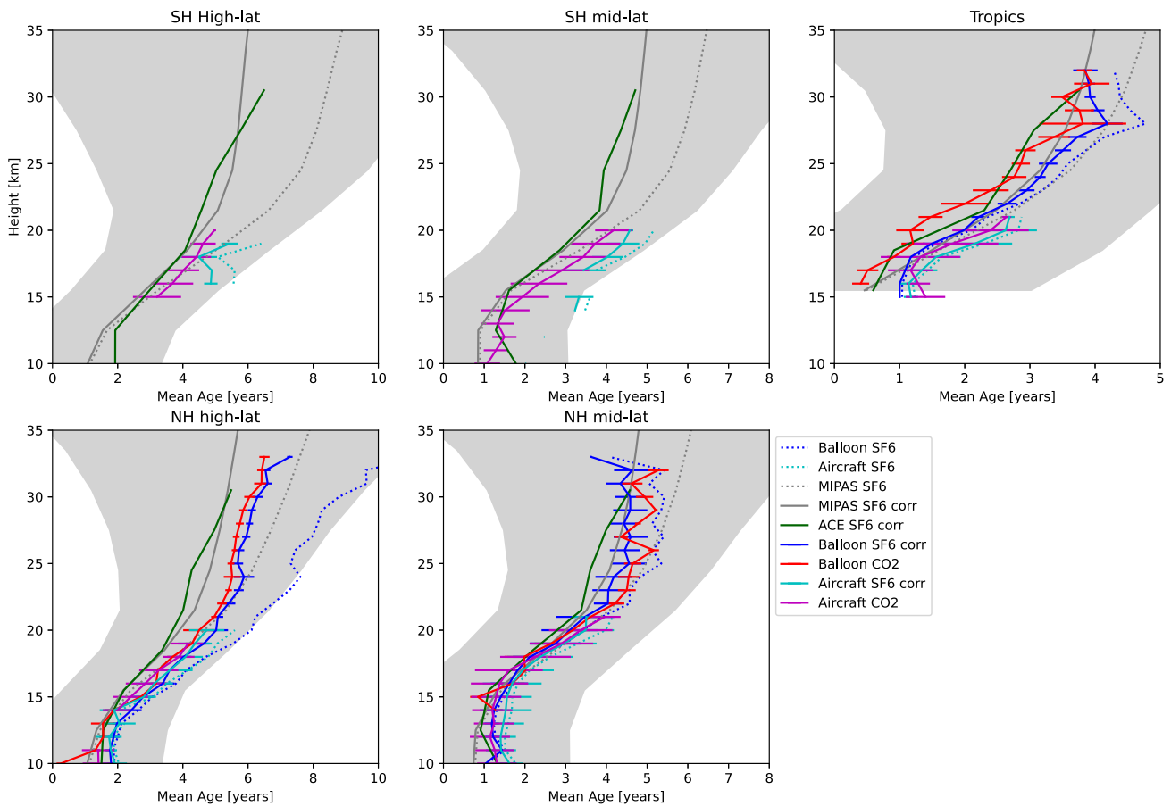
Figure 6. Mean age profiles averaged over high-latitudes ( 90^{\circ} – 60^{\circ} ), mid-latitudes ( 60^{\circ} – 30^{\circ} ) of each hemisphere, and tropics ( -30^{\circ} to 30^{\circ} ) from \text{SF}_6 satellite data (MIPAS, gray dashed line uncorrected mean, solid line sink-corrected mean, and gray shading displays range of \pm 1 standard deviation of the sink-corrected data) and from ACE (darkgreen, shown is only the sink-corrected mean) and averaged over available balloon flights (blue dotted: \text{SF}_6 mean ages; blue solid: \text{SF}_6 mean ages with the sink correction applied; red: \text{CO}_2 mean ages) and averaged over available aircraft flights (light-blue dotted: \text{SF}_6 mean ages; light-blue solid: \text{SF}_6 mean ages with the sink correction applied; magenta: \text{CO}_2 mean ages).
