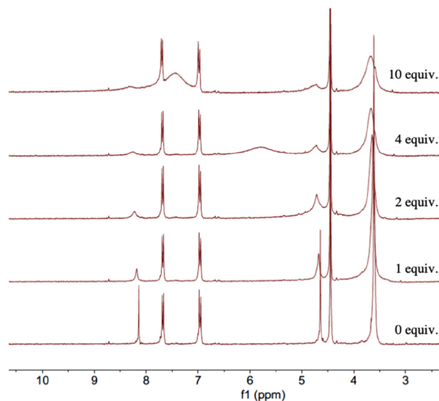
Fig. 16 ^1\text{H} NMR spectra (300 MHz) of compound 8 with 5 equiv. of \text{KPF}_6 and TFA (0–10 equiv.) in \text{CD}_3\text{CN} at 25 ^\circ\text{C} .
