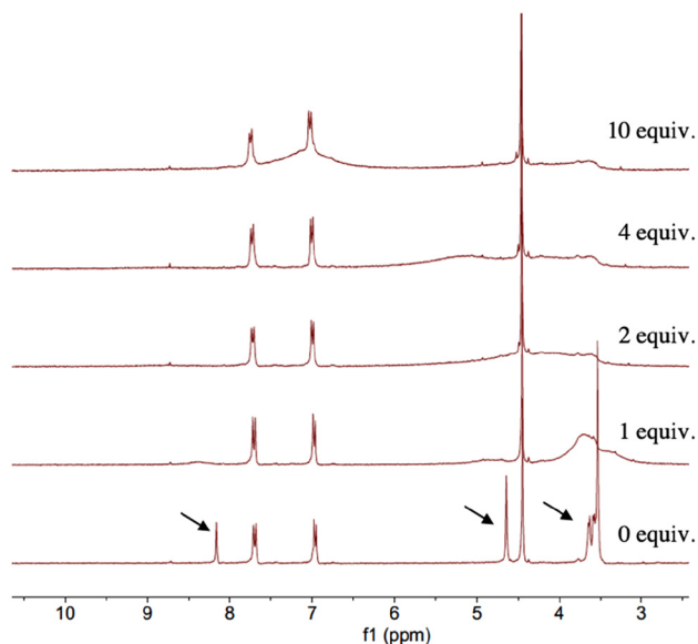
Fig. 14 ^1\text{H} NMR spectra (300 MHz) of compound 8 with TFA (0–10 equiv.) in \text{CD}_3\text{CN} at 25 ^\circ\text{C} . Arrows indicate signals corresponding to the triazole-PEG fragment.
