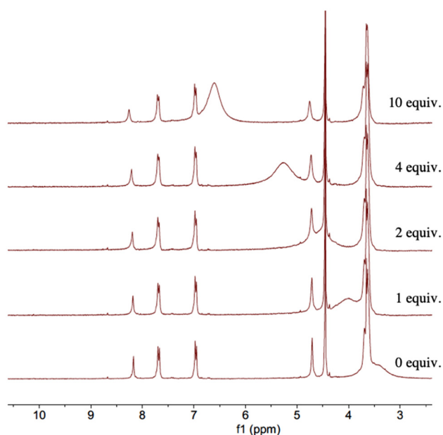
Fig. 15 ^1\text{H} NMR spectra (300 MHz) of compound 8 with 5 equiv. of \text{NaPF}_6 and TFA (0–10 equiv.) in \text{CD}_3\text{CN} at 25 ^\circ\text{C} .
