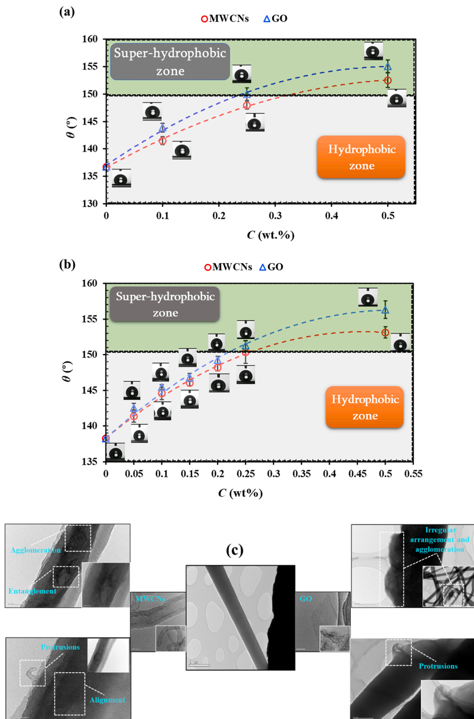
Fig. 3. Water contact angles ( \theta ) at the surfaces of SL-MM-ENMs prepared from LMPVDF (a) and HMPVDF (b) solutions with different contents of MWCNs and GO, and TEM images showing different arrangements of MWCNs and GO in the electrospun nanofiber (c).
