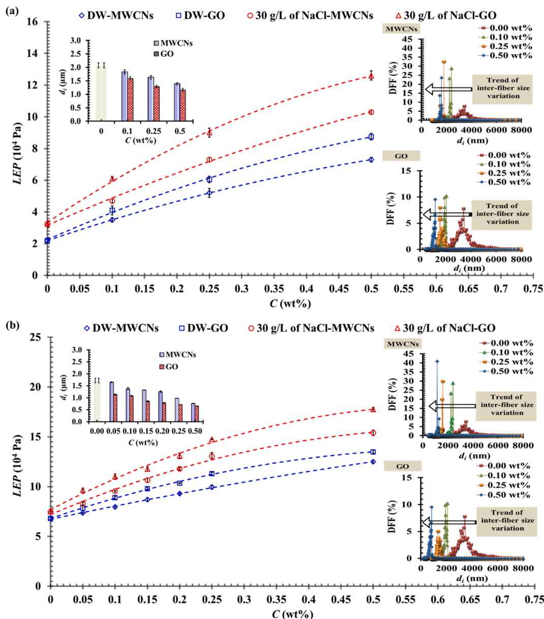
Fig. 5. Liquid Entry Pressure (LEP) values for distilled water and a 30 g/L NaCl aqueous solution as a function of the contents of MWCNs and GO for LMPVDF (a) and HMPVDF (b) SL-MM-ENMs. The right-hand insets show the distribution of the inter-fiber space and the left-hand insets show the variation of the mean inter-fiber space ( d_f ) with the nanofiller concentration.
