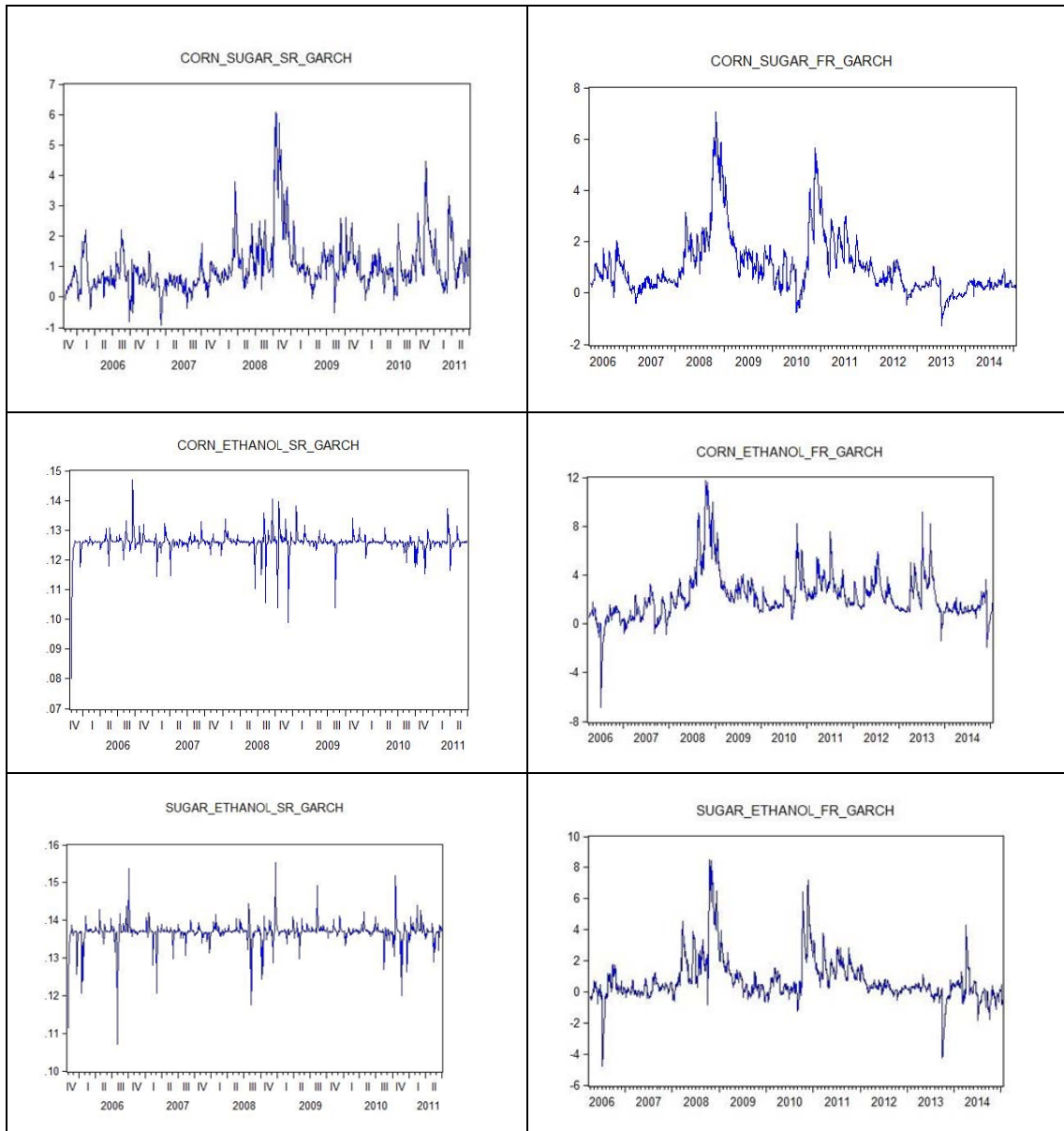
Figure 8 Conditional volatility for Corn & Sugarcane, Corn & Ethanol Sugarcane & Ethanol Spot and Futures Returns
