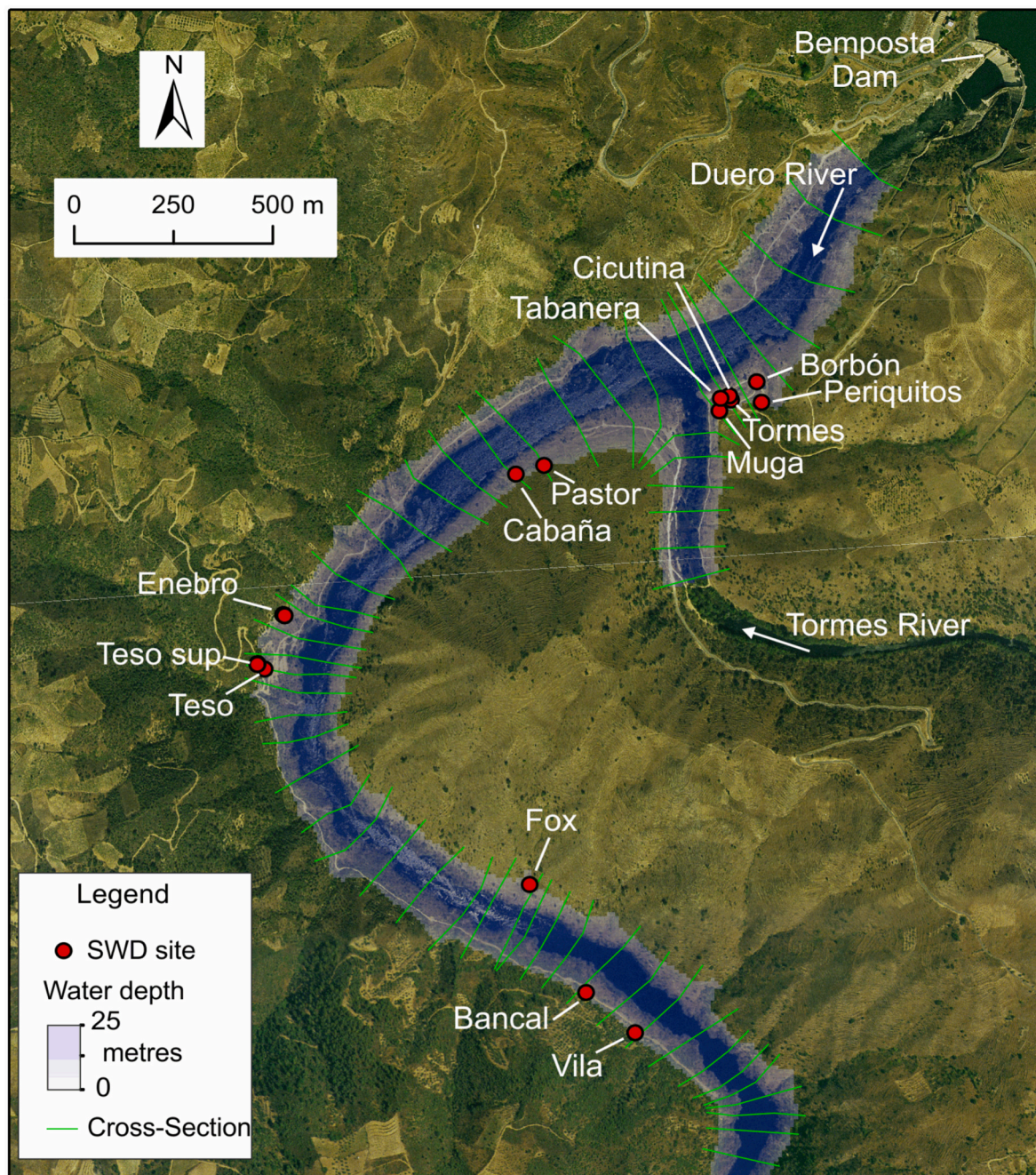
Fig. 3. Orthophotograph of the Bemposta reach (year 2017) showing the locations of the stratigraphic profiles described in the text and the valley cross-sections used in the one-dimensional hydraulic model (HEC-RAS). The cross sections are presented on the 2 m grid DTM generated from Lidar data (provided by the Spanish National Geographic Institute (IGN; https://www.ign.es , last accessed: 4 May 2023) in ArcGIS. The water depths correspond to a modelled discharge of 11,000 m 3 /s.
