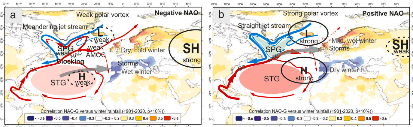
Fig. 12. Main components of the atmospheric and ocean circulation during periods of negative (a) positive (b) and NAO phases. The yellow and blue background on continental regions shows the correlation ( r^2 ) between NAO-Gibraltar index and the precipitation from CRU TS4.06 precipitation dataset (wrt: 1901–2020, p < 10\% ). Correlations are averaged-computed for November–March in order to match with the main flood season in the Duero basin. Atmospheric circulation centers of actions in the North Atlantic Basin and Europe (Icelandic and Azores pressure cells, and Siberian High-SH) are shown in black lines. Continuous lines show strong conditions of Low and High pressure centers and dashed lines indicates weak pressure conditions. Grey thick transparent arrow shows general vector of the vertically integrated moisture transport during negative NAO index (a) and positive NAO index (b) after Hurrell (1995) and Hurrell et al. (2003). Modern surface water hydrography of the North Atlantic currents are modified from Schott et al. (2004) and Repschläger et al. (2017). Warm surface currents are shown by red arrows, and cold currents are shown by blue arrows. Line thickness reflects relative flow rate. Legend: G.S., Gulf; N.A.C., North Atlantic Current; AMOC, Atlantic Meridional Overturning Circulation; SPG, North Atlantic Subpolar Gyre; STG, Subtropical Gyre.
