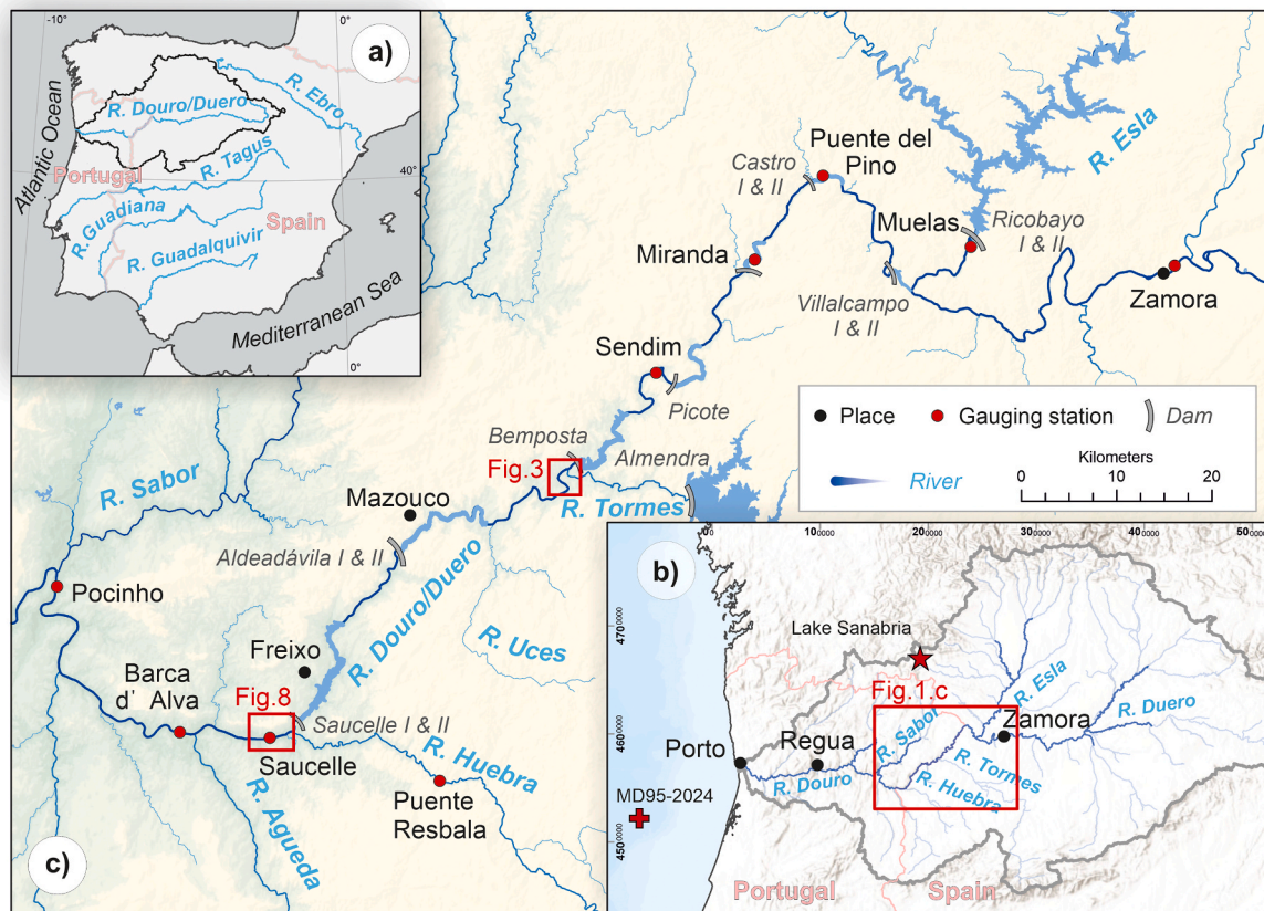
Fig. 1. a) Location map of the Duero River catchment within the Iberian Peninsula and the other major river basins draining to the Atlantic Ocean. b) Relief map of the NW Iberian Peninsula and the boundary of the Duero catchment, the main river network and cities. The rectangle shows the location of (c). c) Hillshade map of the international section of the Duero/Douro River along the border between Spain and Portugal. The study reaches are located (1) downstream of the Bemposta dam and (2) downstream of the Saucelle dam. Also shown are the locations of gauge stations and sites with important hydroclimatic proxy records, Lake Sanabria (Jambrina-Enriquez et al., 2014, 2016) and marine core MD95-2040 at the Iberian margin (de Abreu et al., 2003).
