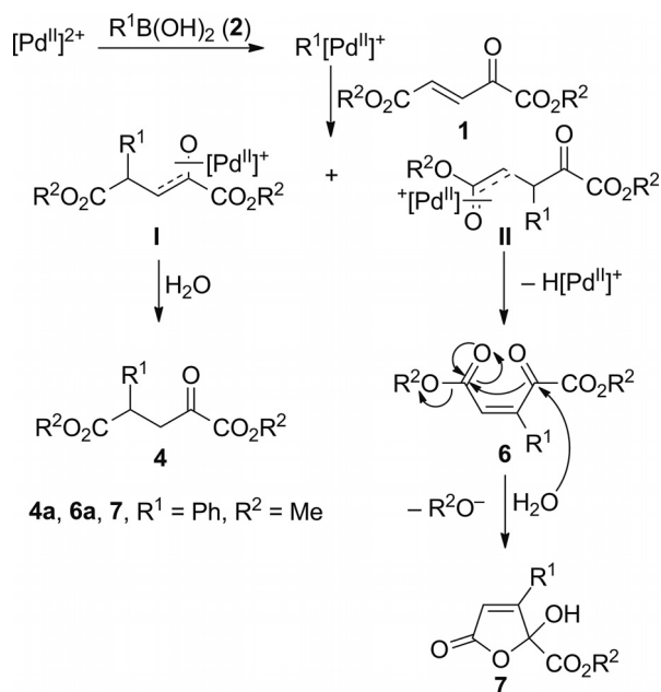
Scheme 2. Reaction course.
