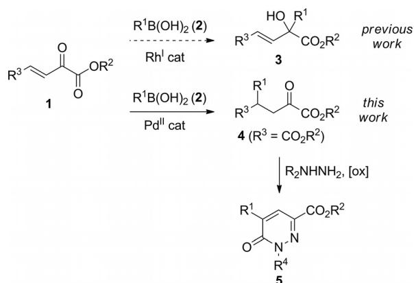
Scheme 1. Conjugate addition of boronic acids to \alpha,\beta -unsaturated \alpha -keto esters.
