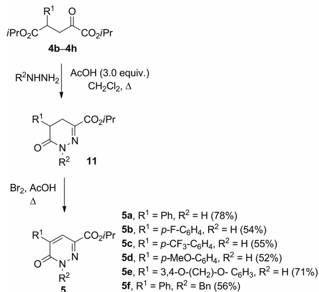
Scheme 3. Synthesis of pyridazin-3(2 H )-ones 5 .
