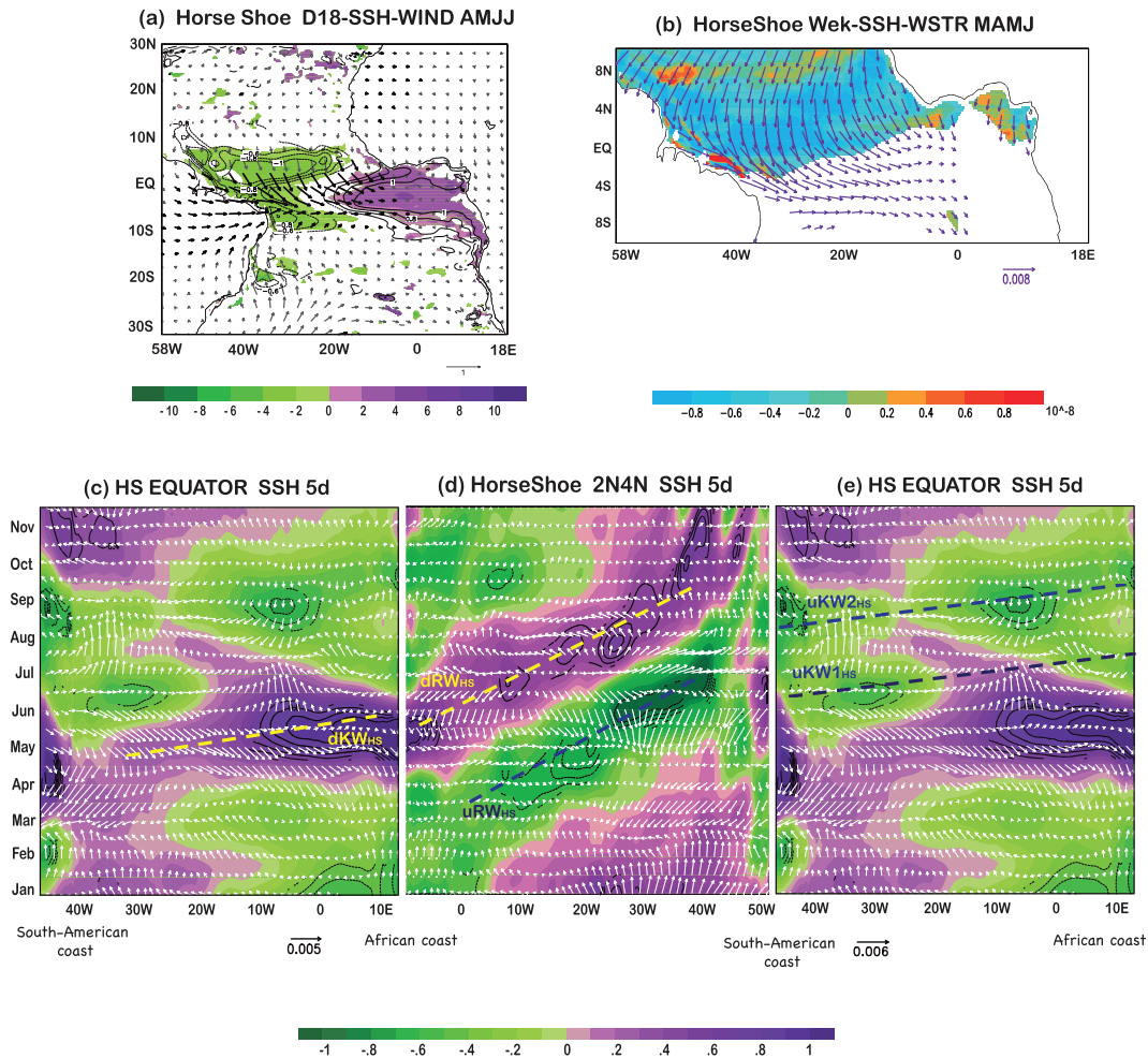
Figure 4. Wave activity involved in the development of HS. (a) Regression of the anomalous observed surface wind (vectors, m/s), thermocline depth (shaded, m) and SSH (contour, cm) in AMJJ onto the PC of the HS fixed during boreal summer (JJAS). Significant values exceeding 95% confidence level according to a t-test are shown in shaded, black and purple contours and vectors. (b) Regressed wind stress (vectors, N/m^2 ) and wind stress curl (shaded, N/m^3 ) in MAMJ onto the PC of HS fixed in boreal summer (JJAS). Significant values are shown in shaded and purple vectors. (c-e) Time-longitude diagrams of the regressed 5-day SSH anomalies (shaded, cm) and wind stress (vectors, N/m^2 ) from January to December onto the PC of HS. Significant values exceeding 95% according to a t-test are shown in black contours. Downwelling (upwelling) KW and RW are indicated by yellow (blue) arrows.
