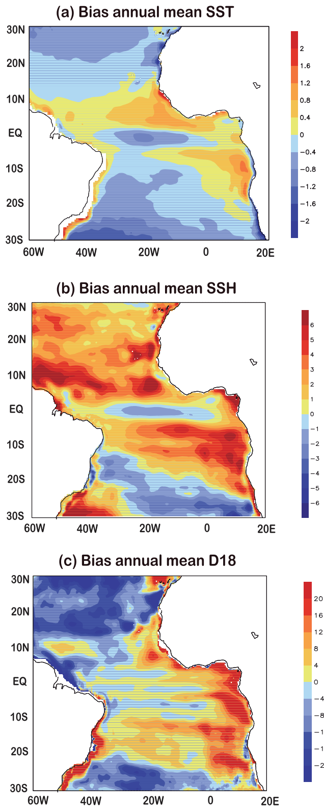
Figure 1. Validation of INTER simulation. Bias of the annual SST(a), SSH (b) and thermocline depth (D18, c) of INTER simulation with respect to SODA reanalysis for the period 1960-2008.
