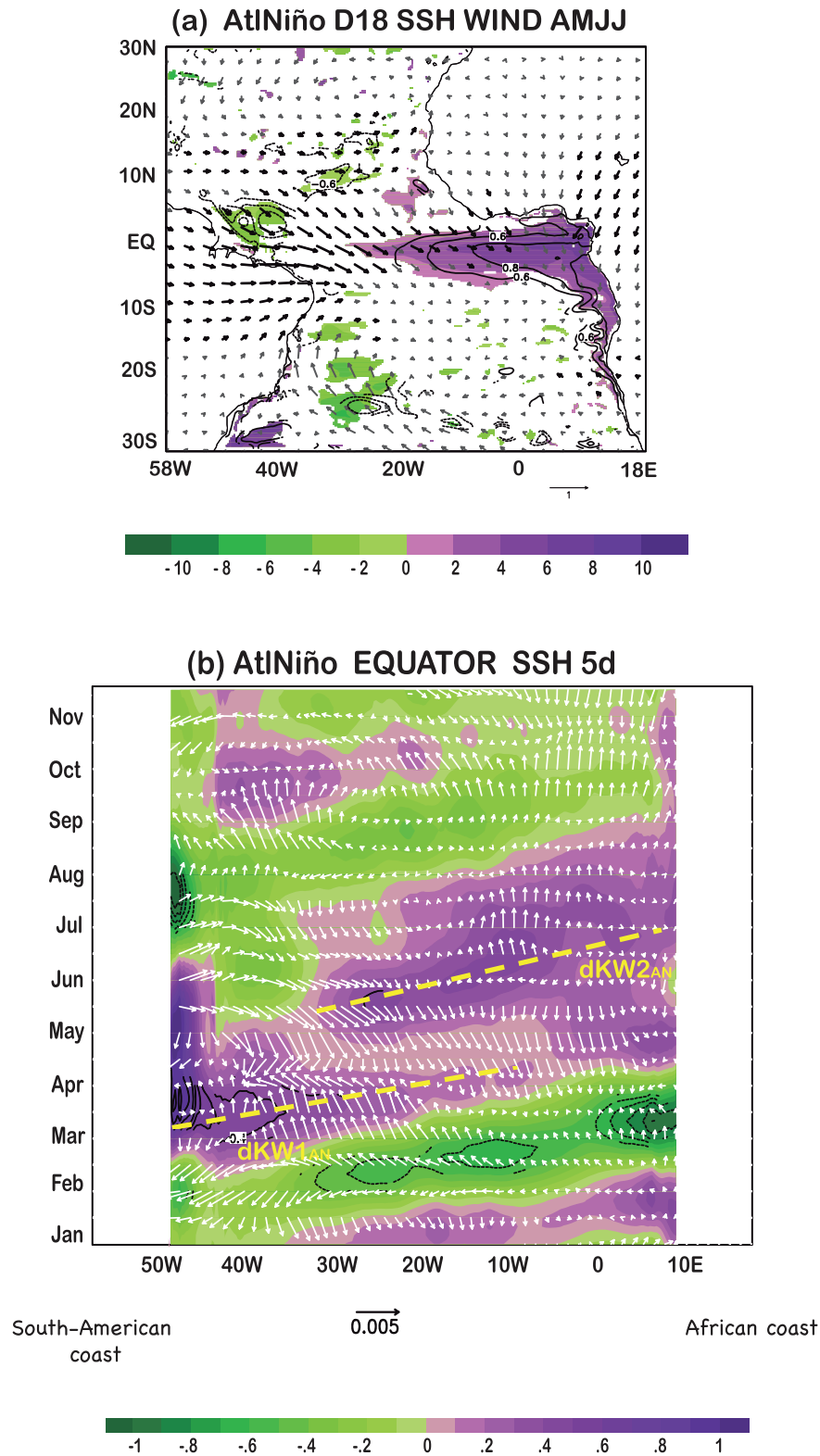
Figure 3. Wave activity involved in the development of Atlantic Niño. (a) Regression of the anomalous observed surface wind (vectors, m/s), thermocline depth (shaded, m) and SSH (contour, cm) in AMJJ onto the PC of Atlantic Niño fixed during boreal summer (JJAS). Significant values exceeding 95% confidence level according to a t-test are shown in shaded, black contours and vectors. (b) Time-longitude diagrams at the equator of the regressed 5-day SSH anomalies (shaded, cm) and wind stress (vectors, N/m^2 ) from January to December onto the PC of Atlantic Niño. Significant values exceeding 95% according to a t-test are shown in black contours. Downwelling KW are indicated by yellow arrows.
