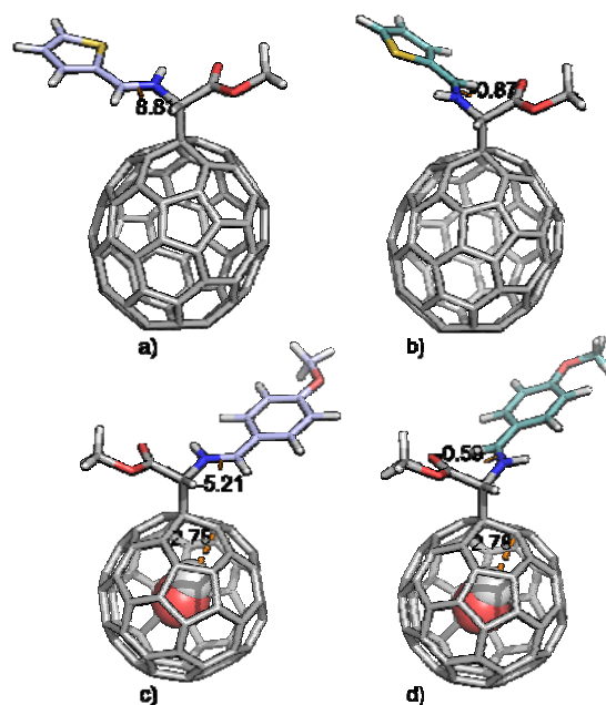
Figure 4. DFT optimized cis-trans intermediates for: a) INT(2S,5S)- cis -3, b) INT(2S,5R)- trans -3, c) INT(2S,5S)- cis -5a, and d) INT(2S,5R)- trans -5a. H_{H_2O}-C_{full} distance in angstroms and \angle CNCH dihedral angle in degrees.
