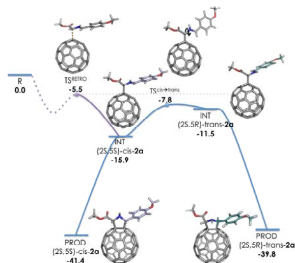
Figure 3. DFT mechanism for the cis-trans 2a isomerization (represented using a blue line) and retro-Prato process (in purple). All energies are expressed in kcal/mol.
