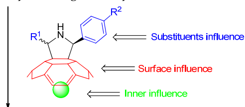
Figure 1. “Three levels” approach that may influence the stereochemical result of the cis/trans isomerization in fulleropyrrolidines.
