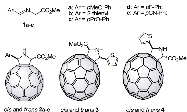
Figure 2. Optically pure [60] and [70]fulleropyrrolidines
