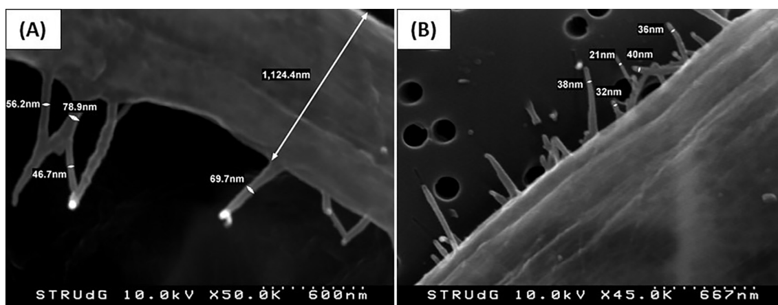
Fig. 2. FE-SEM observation of LCMNF 1 (A) and LCMNF 4 (B).
