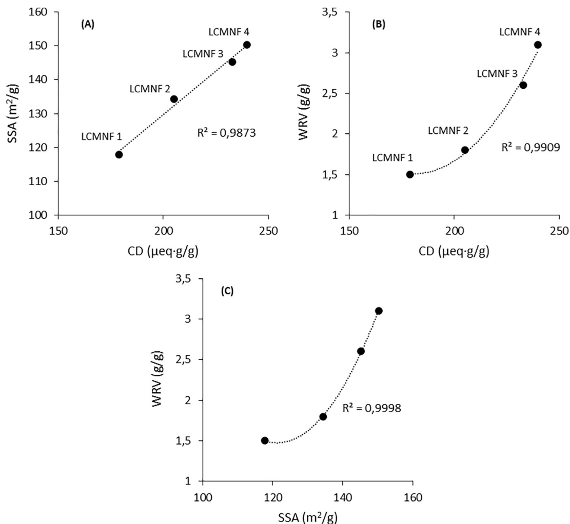
Fig. 3. Evolution of the SSA CR (A) and WRV (B) with the CD, and WRV with the SSA CR of the LCMNF (C).
