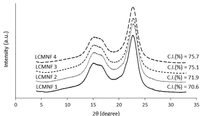
Fig. 4. XRD analysis of the LCMNF.
