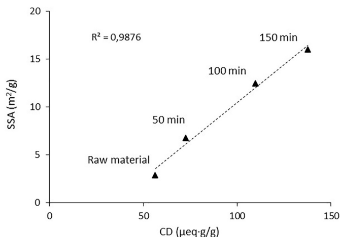
Fig. 1. Evolution of SSA and CD at different processing times in the Valley beater.
