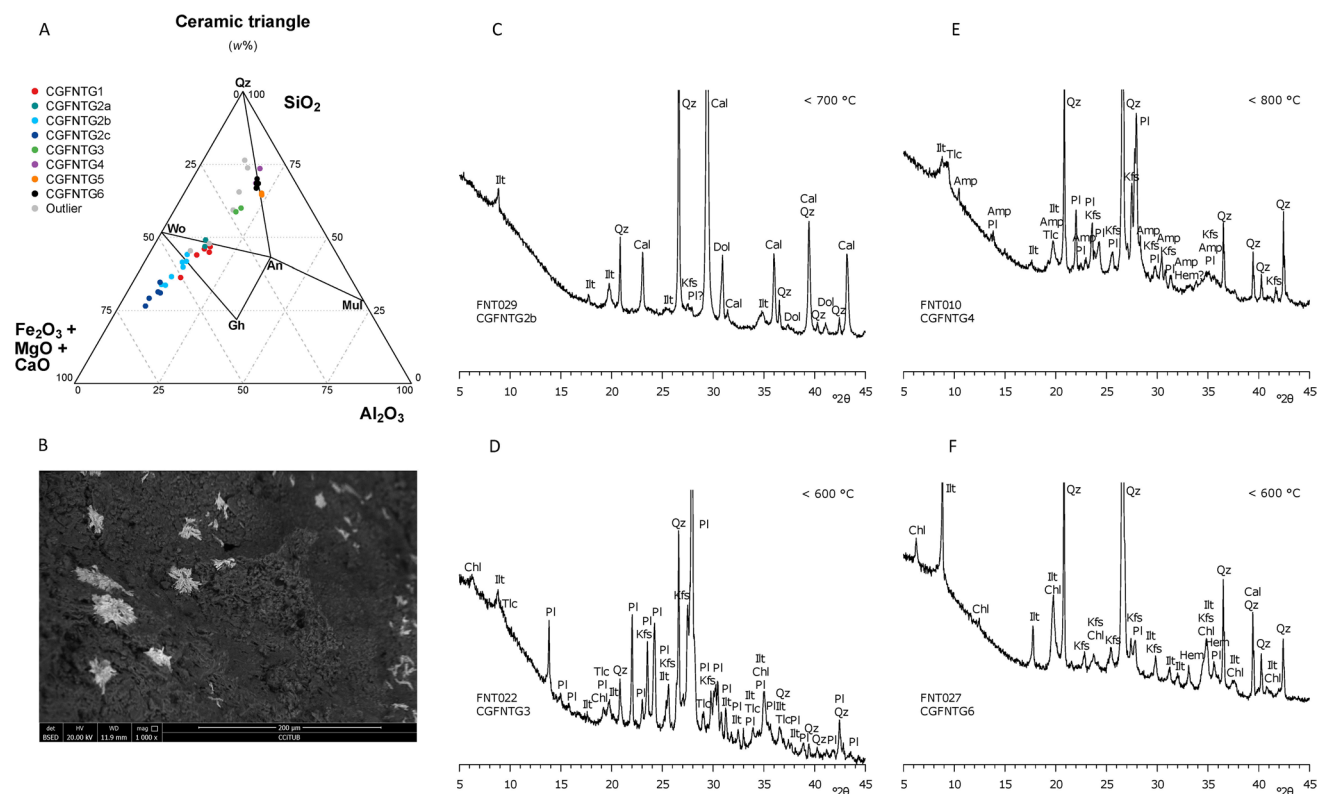
Fig. 9 A: Phase diagram of the ternary system (Fe 2 O 3 + MgO + CaO)-Al 2 O 3 -SiO 2 (ceramic triangle) showing the situation of the individuals analysed. B: Photomicrograph by SEM of the individual FNT023 (group CGFNTG2a) using the backscattered detector showing authigenic crystals of baryte. C to F: XRD patterns for the categories of association of crystalline phases as detected by XRD. C: individual FNT029 XRD pattern CGFNTG2b-1. D: individual
