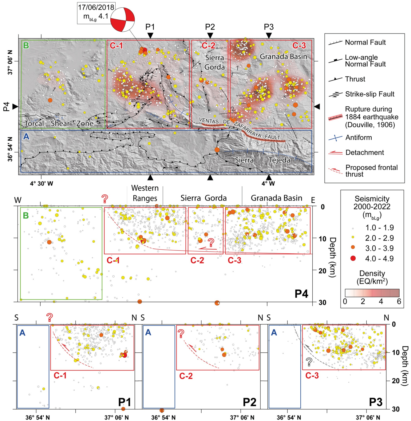
Figure 3. Map of the relocated seismicity (Table S1), including the projected seismicity on a W–E profile and three N–S cross-sections. The zones described in the results section are depicted in blue (a), green (b), and red (c). The maps show the earthquake focal mechanism associated with the highest magnitude event since the year 2000. The P4 profile includes all the relocated seismicity data. The P1, P2, and P3 profiles illustrate the seismicity in C-1, C-2, and C-3 red boxes, respectively, and their southern continuation.
