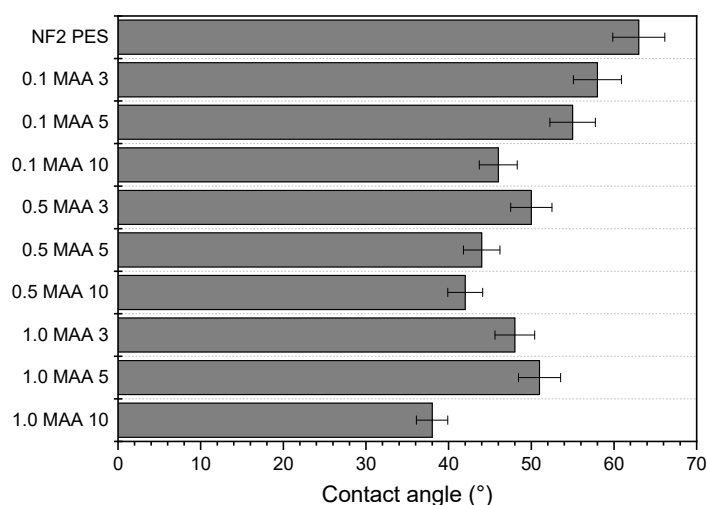
Figure 3. Water contact angle of the unmodified and UV-grafted membranes.
