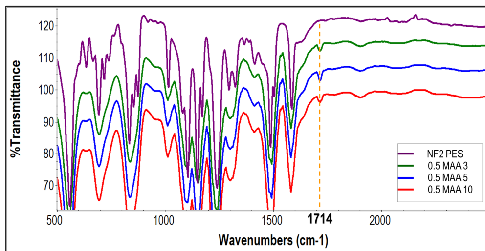
Figure 6. FTIR-ATR spectra of the unmodified NF2 PES and UV–grafted membranes 0.5 MAA3, 0.5 MAA5 and 0.5 MAA10.
