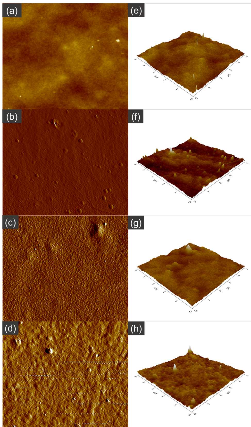
Figure 8. AFM images ( 5\ \mu\text{m} \times 5\ \mu\text{m} ) of the top surface of the NF2 PES membrane (a,e) and UV-grafted membranes 0.1 MAA3 (b,f), 0.5 MAA3 (c,g) and 1.0 MAA3 (d,h).
