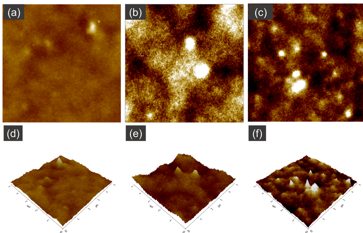
Figure 9. AFM images ( 5\ \mu\text{m} \times 5\ \mu\text{m} ) of the top surface of the modified membranes 0.5 MAA3 (a,d), 0.5 MAA5 (b,e) and 0.5 MAA10 (c,f).
