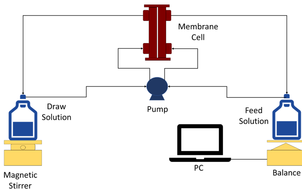
Figure 1. Schematic diagram of FO system.
