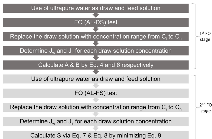
Figure 2. Flow chart of the two-stage non-pressurized method.
