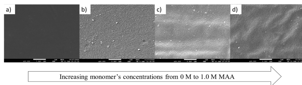
Figure 12. FESEM images ( 20,000\times magnification) of the top surface of the membranes: (a) NF2PES, (b) 0.1 MAA3, (c) 0.5 MAA3 and (d) 1.0 MAA3.
