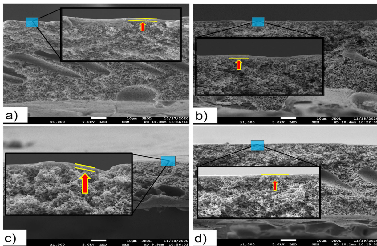
Figure 10. FESEM images ( 1000\times magnification) of the membranes: (a) cross section of NF2 PES, (b) cross section of 0.5 MAA3, (c) cross section of 0.5 MAA5, (d) cross section of 0.5 MAA10.
