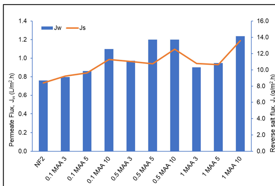
Figure 13. Water permeate flux ( J_w ) and reverse salt flux ( J_s ) of the unmodified NF2 PES membrane and the UV-grafted membranes under different modification conditions, with 1 M NaCl draw solution and DI water as feed.
