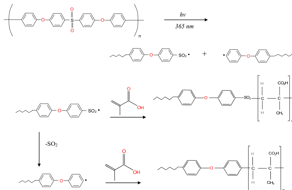
Figure 5. UV–photochemical grafting modification of polyether(sulfone) with methacrylic acid.
