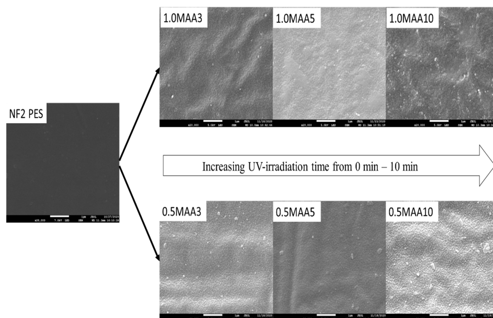
Figure 11. FESEM images ( 20,000\times magnification) of the top membrane surface showing the effect of UV irradiation time.
