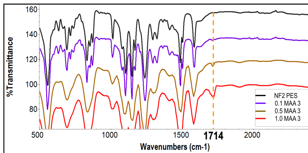
Figure 4. FTIR-ATR spectra of the unmodified NF2 PES and UV-grafted membranes 0.1 MAA3, 0.5 MAA3 and 1.0 MAA3.
