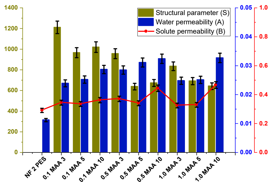
Figure 14. Structural parameter (S), water permeability (A) and salt permeability (B) of the UV-grafted membranes.
