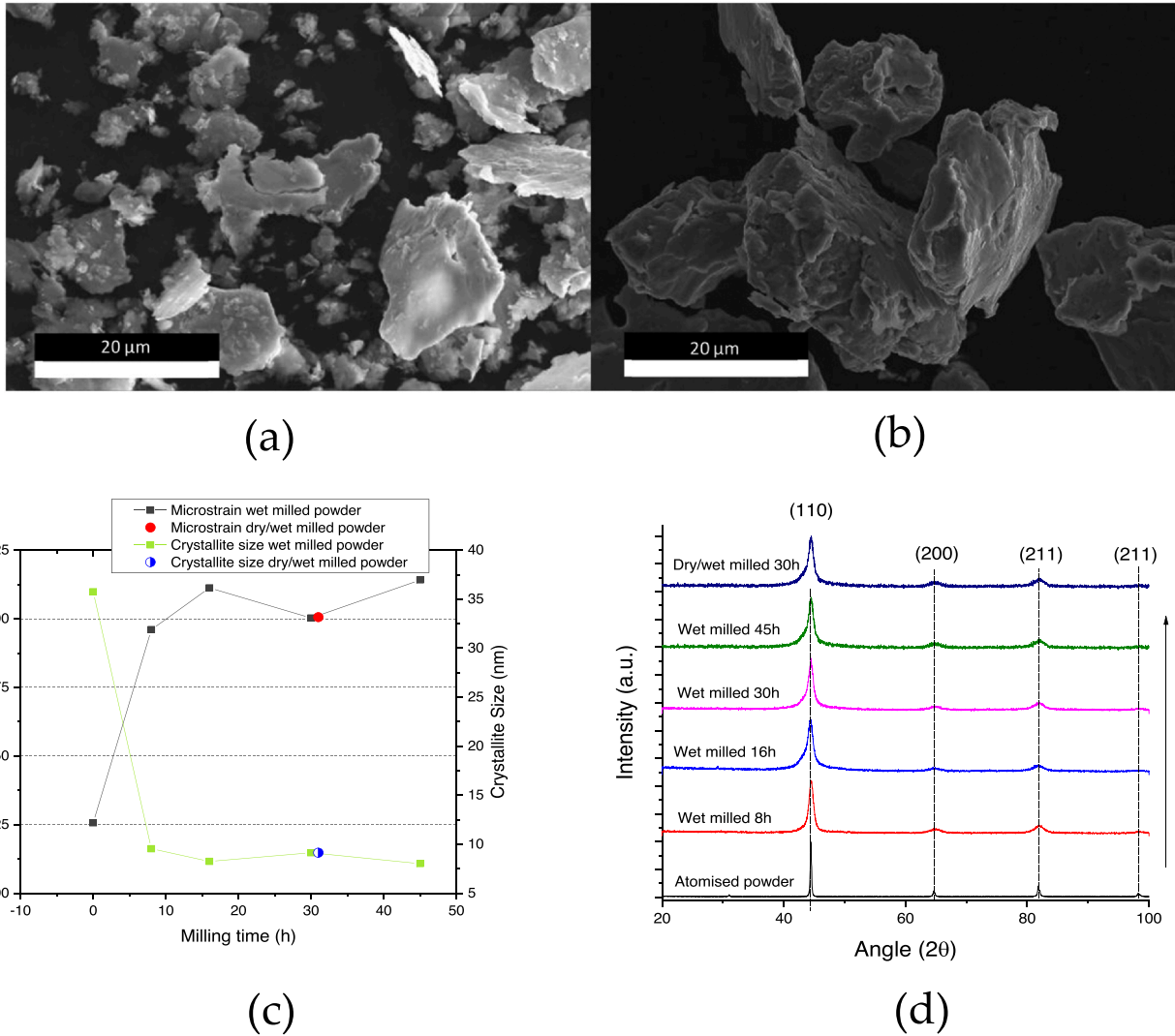
Fig. 1. (a) SE-SEM image of Wet milled powder for 45 h; (b) SE-SEM image of Dry/Wet milled powder for 30 h; (c) Microstrain and Crystallite size evolution versus milling time and (d) XRD patterns of all the specimens at the selected milling times.
