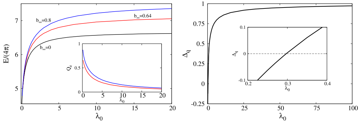
Fig. 4. Left panel: The energy E and the electric charge Q_e are shown vs. the coupling constant \lambda_0 for SO(2) gauged Skyrmions in 3 + 1 dimensions, with n = 1 , \lambda_1 = \lambda_2 = \lambda_3 = 1 , and several values of b_\infty . Right panel: The relative difference \Delta_q = (q_G - q_W)/(q_G + q_W) of the individual contributions to the topological charge q = q_G + q_W = 1 is shown vs. the coupling constant \lambda_0 for the same solutions.
