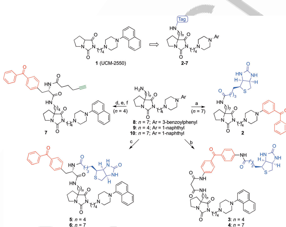
Scheme 1. Design and synthesis of probes for serotonin 5-HT 1A R: a) biotin, DCC, HOBT, DMAP, DMF, RT, 39%; b) 3-oxo-3-((4-[4-(biotinylamino)benzoyl]phenyl)amino)propanoic acid ( 11 ), EDC, HOBT, DMF, DCM, RT, 15–36%; c) 4-benzoyl- N -biotinyl-L-phenylalanine ( 12 ), EDC, HOBT, DMF, DCM, RT, 20–46%; d) Fmoc-4-benzoyl-L-phenylalanine, EDC, HOBT, DMF, DCM, RT, 80%; e) piperidine, DCM, 0 °C, 75%; f) 5-hexynoic acid, DCC, DMAP, DCM, RT, 53%. DCC = N,N -dicyclohexylcarbodiimide; DCM = dichloromethane; DMAP = 4-dimethylaminopyridine; EDC = N '-(3-dimethylaminopropyl)- N -ethylcarbodiimide; Fmoc = 9-fluorenylmethoxycarbonyl; HOBT = 1-hydroxybenzotriazole.
