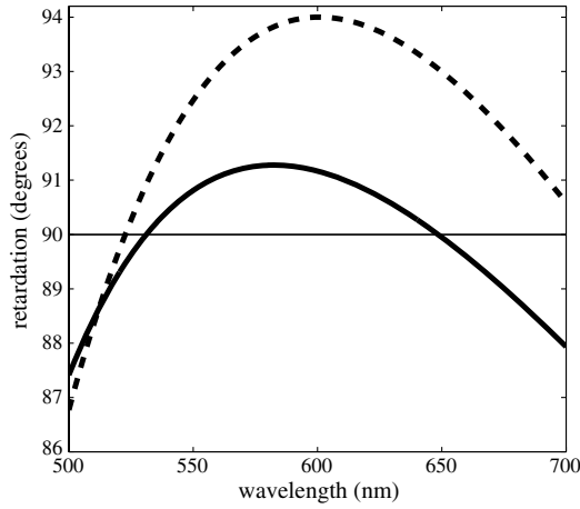
Fig. 2. Optimal overall retardation of the system for a Gaussian and plane spectrum (continuous curve) centered at \lambda_0 = 600 nm and a width \delta\lambda = 100 nm, with wavelength [500,700] nm. Both curves are coincident. A previous result of overall retardation is shown with a dashed curve [8].
