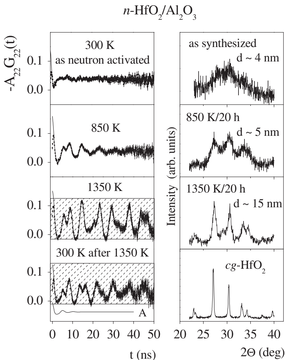
FIG. 7. PAC spectra of ^{181}\text{Ta} in \text{Al}_2\text{O}_3 -coated nanoparticles of \text{HfO}_2 (powder sample in vacuum) at different temperatures (left-hand column), and room temperature x-ray diffraction spectra of n\text{-HfO}_2/\text{Al}_2\text{O}_3 after synthesis and after annealing at 850 and 1350 K, respectively (right-hand column). The height of the striped area is a measure of the monoclinic fraction at 1350 K. The particle size has been derived from the linewidth of the x-ray reflections. For comparison, the x-ray pattern of commercial \text{cg-HfO}_2 is shown in the bottommost section of the right-hand column.
